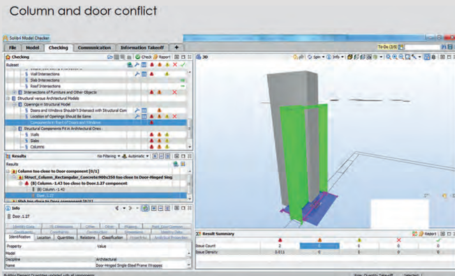
Figure 1–7 Detecting coordination issues in BIM via a model checker by Mitchell Brandtman 5D Quality Surveyors.
