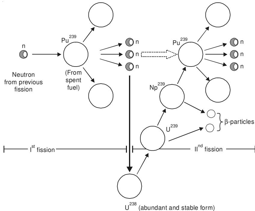
Fig. 12.7. Nuclear fission reaction sequence in breeder reactor. Here plutonium ( \text{Pu}^{239} ) is used as well as produced in abundance
