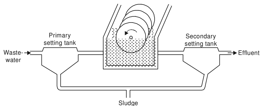
Fig. 12.27. Rotating biological contactor
