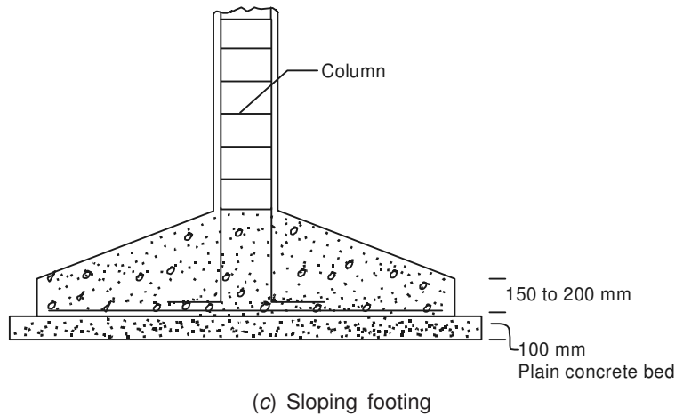
Fig. 4.5. Isolated column footing
