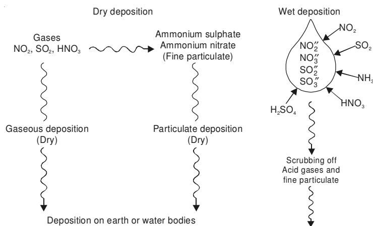
Fig. 10.12. Acid deposition (dry deposition and wet deposition)
