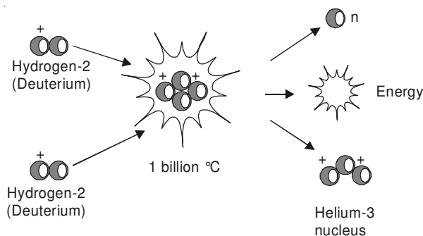
Fig. 12.2. Nuclear fusion reaction between two hydrogen-2 nuclei, which takes place at a very high temperature of 1 billion ^{\circ}\text{C} ; one neutron and one fusion nucleus of helium-3 is formed along with a huge amount of energy
