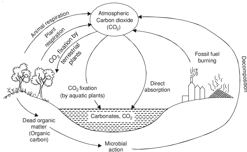
Fig. 10.4. Carbon cycle
