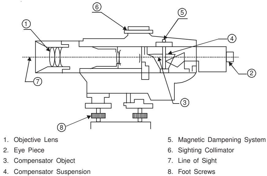
Fig. 7.3. Auto Level—Cross Sectional View.
