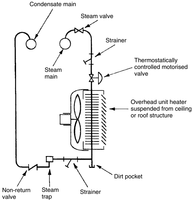
Overhead unit heater connections
