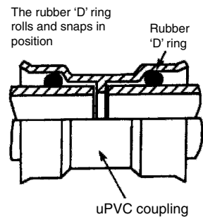
Flexible joint on uPVC pipe
