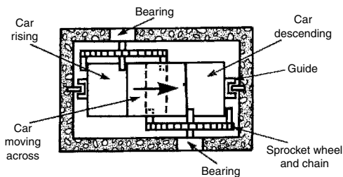
Plan of lift at top changeover
