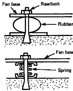
Use of rubber or spring mountings
