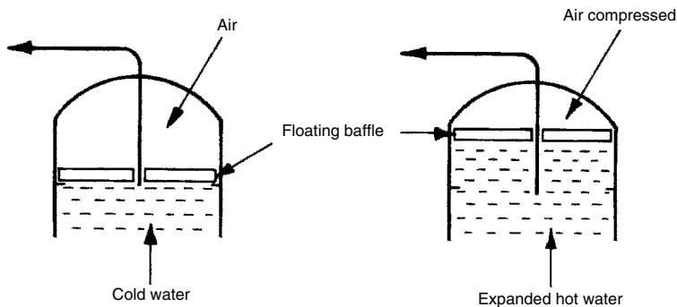
Function of the internal air gap
