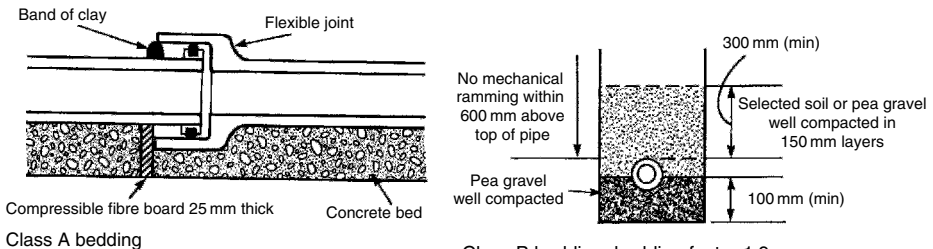
Class B bedding: bedding factor 1.9
