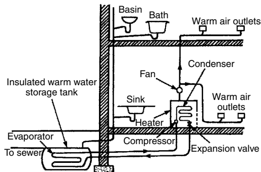
Heat pump used for extracting heat from warm waste water
