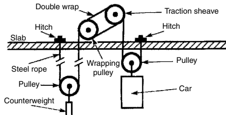
Double wrap 2 : 1 roped (for high speed and medium to heavy duty loads)
