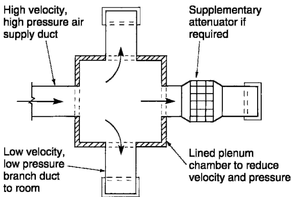
Distribution plenum
