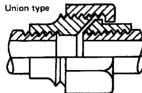
Screwed joints on mild steel pipes
