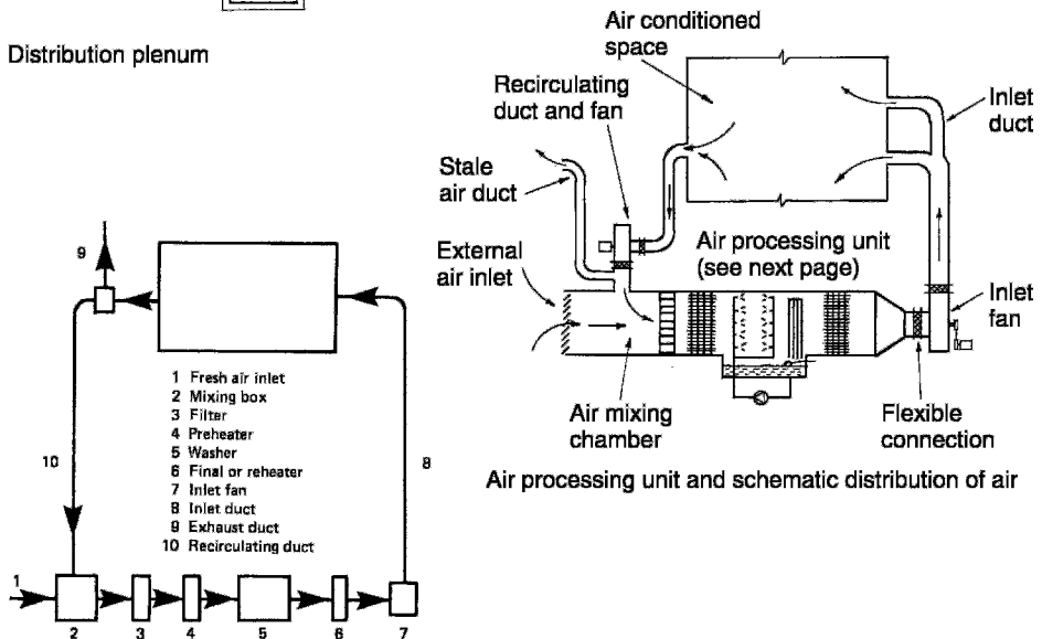
Diagrammatical layout of central plant only system
