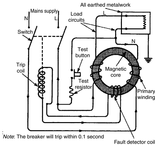
Single-phase RCD
