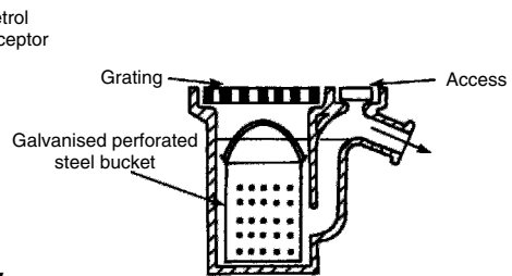
Section of garage gully
