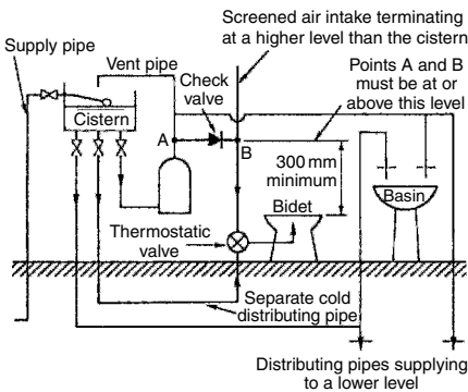
Installation pipework for bidet
