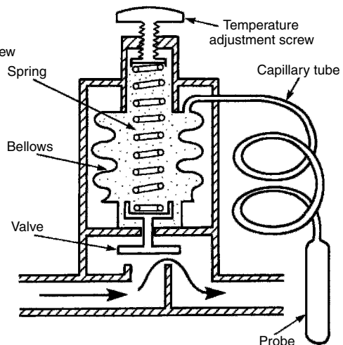
Vapour expansion thermostat
