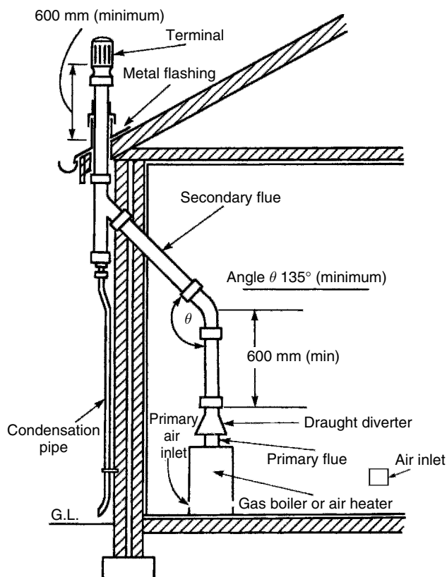
Installation of flue
