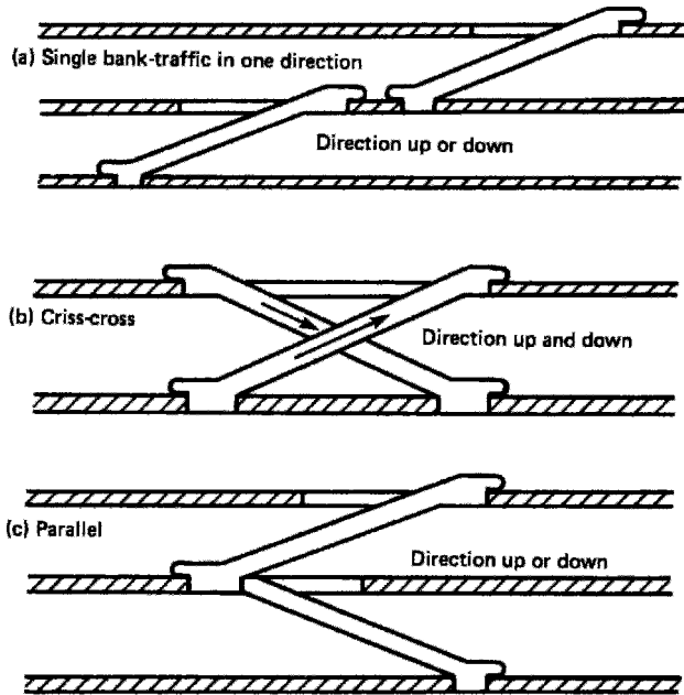
Escalator arrangements
