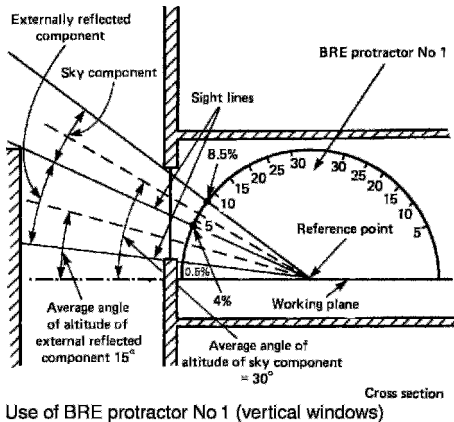
Use of BRE protractor No 1 (vertical windows)
