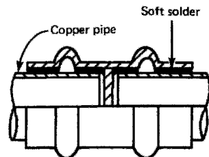
Soft soldered capillary joint on copper pipes
