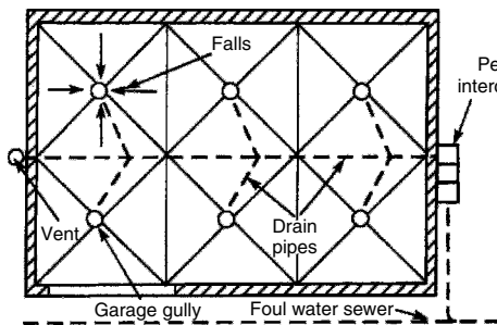
Plan of garage showing drainage
