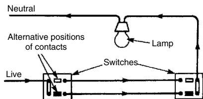
Two-way switching
