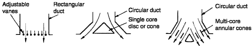
Some types of diffuser (section)
