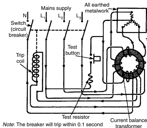
Three-phase RCD
