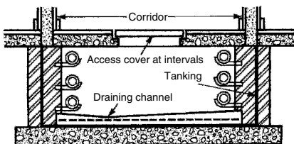
Crawl-way inside a building
