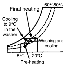
Humidifying by pre-heating, washing and final heating
