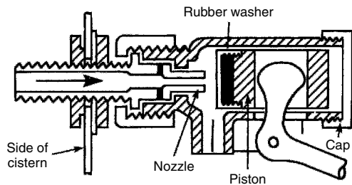
Portsmouth/piston float valve BS 1212-1
