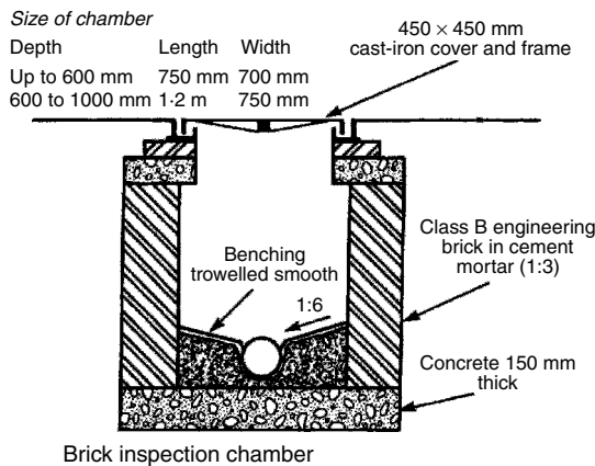
Brick inspection chamber
