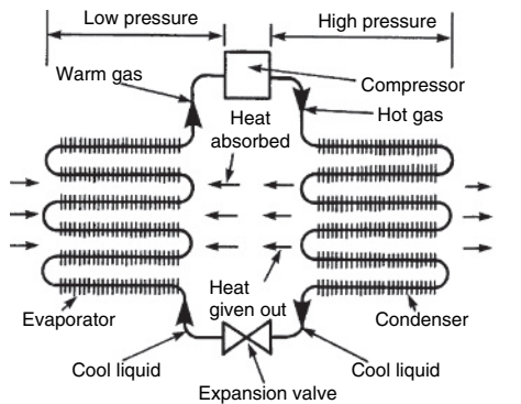
Principles of operation of the heat pump
