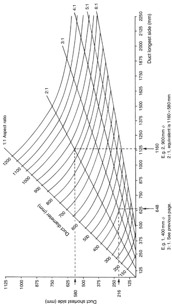
Approximate comparative ducting profiles
