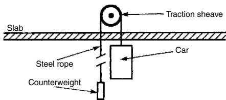
Single wrap 1 : 1 roped
