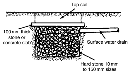
Filled soakaway
