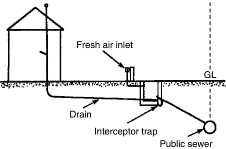
With the use of an interceptor trap
