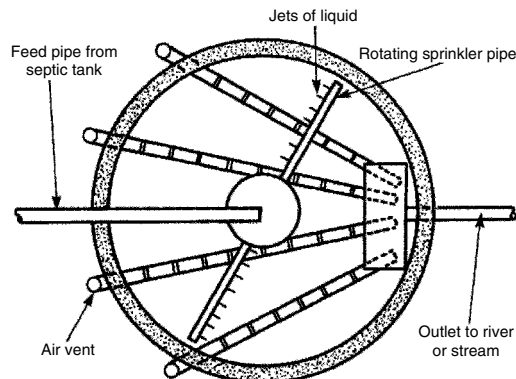
(b) Plan
