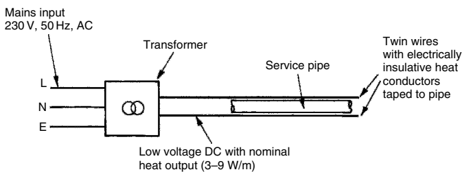
Trace element heating
