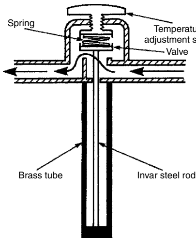
Rod-type thermostat
