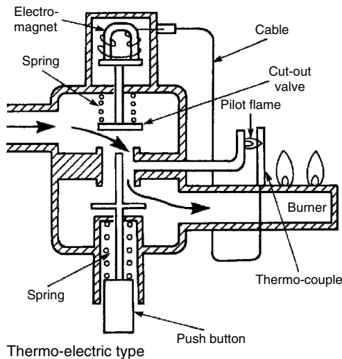
Thermo-electric type
