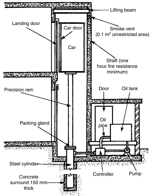
Vertical section
