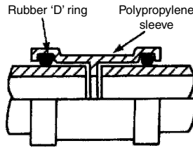
Pipe is lubricated and pushed into the sleeve
