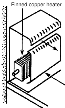
Convector skirting heater
