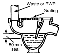
Waste or rainwater gully
