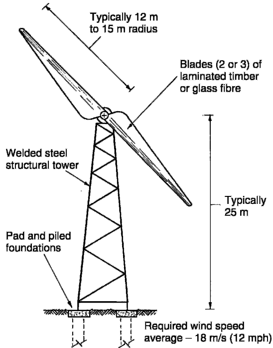
Wind power generator
