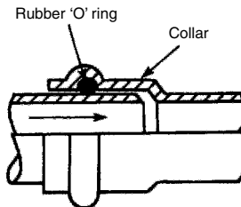
Pipe is lubricated and pushed into collar
