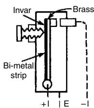
Room thermostat
