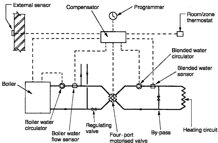
Weather compensated control system
