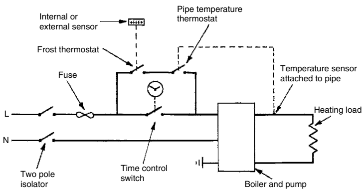
Thermostatic frost protection
