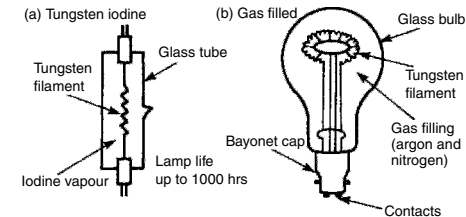
Filament lamps (efficacy = 10–15 lm/W)
