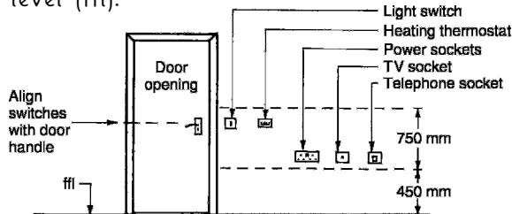
Location of switches and sockets in a dwelling
