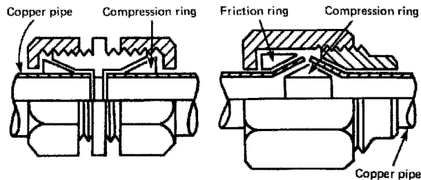
Non-manipulative compression joint on copper pipes
