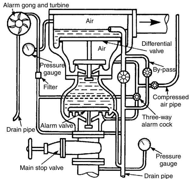
Dry pipe or alternate wet-and-dry pipe controls
