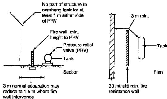
Storage tank location
