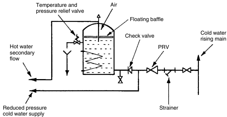
Unvented hwsc incorporating an air gap
