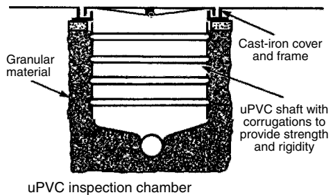
uPVC inspection chamber
