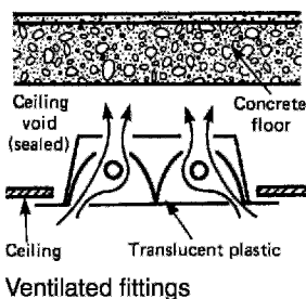
Fittings used for fluorescent lamps
