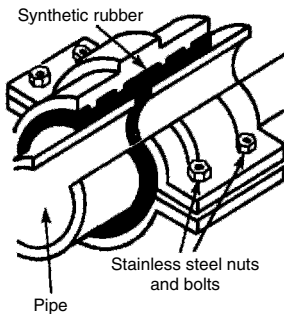
Flexible joint on cast-iron pipe
