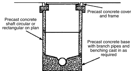
Precast concrete inspection chamber
