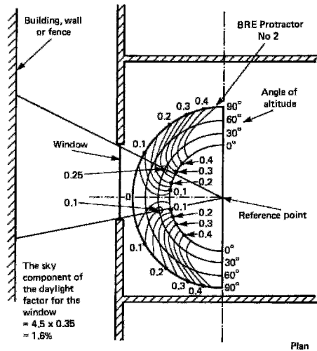
Use of BRE protractor No 2 (vertical windows)
