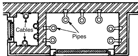
Built-out for large pipes and cables
