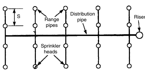
Two-end centre with end feed pipe
