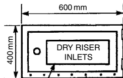
(b) Front view of Fire Brigade inlet box
