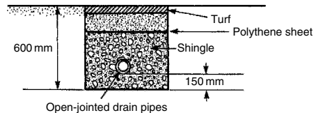
Subsoil irrigation pipe trench
