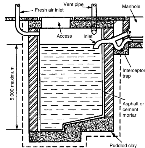
Brick cesspool
