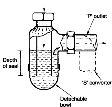
Bottle trap
