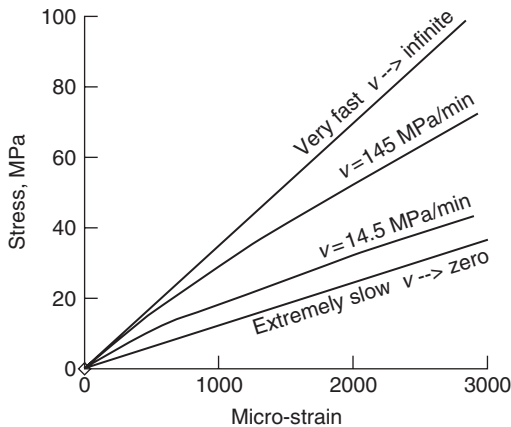
Figure 13-6 Effect of stress rate on the stress strain diagram.
