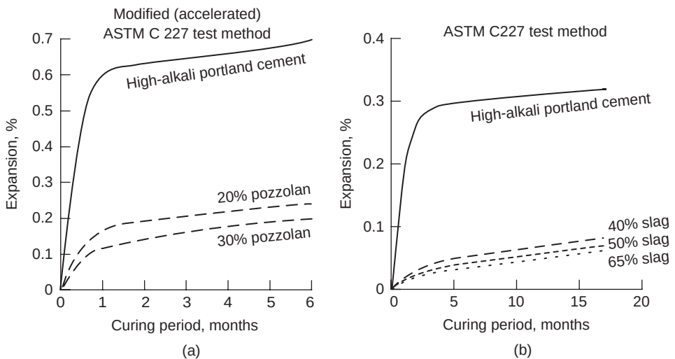
Figure 6-18 Influence of pozzolan or slag addition on alkali-aggregate expansion. [(a) From Mehta, P.K., Cem. Concr. Res. , Vol. 11, No. 4, Copyright 1981, Pergamon Press, New York; (b), reprinted with permission from Hogan, F.J. and J.M. Meusel, Cem. Concr. Aggregates , Vol. 3, No. 1, 1981, ASTM, Philadelphia, PA.]
