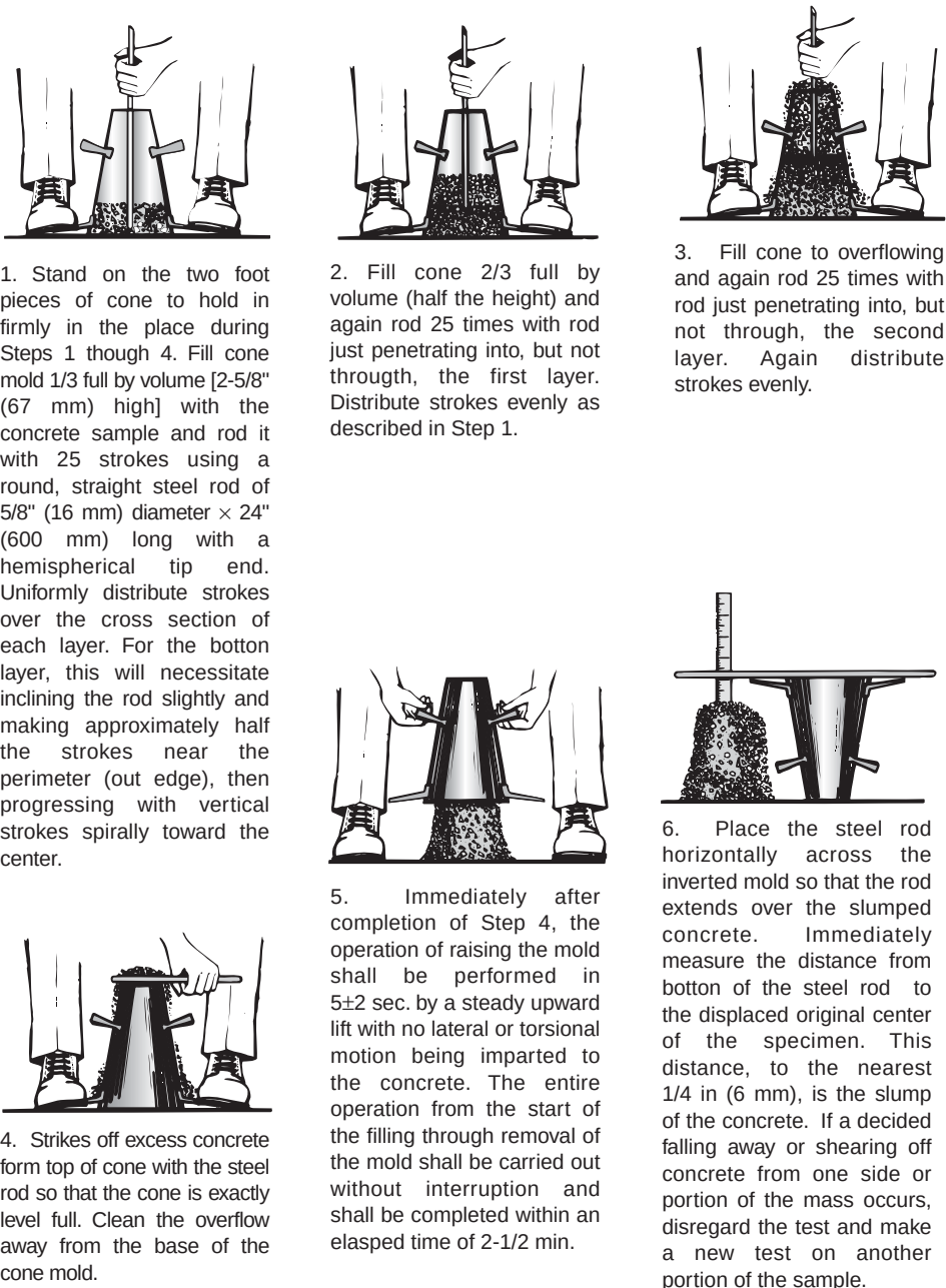
Figure 10-5 Sequence of steps in the slump test procedure.
