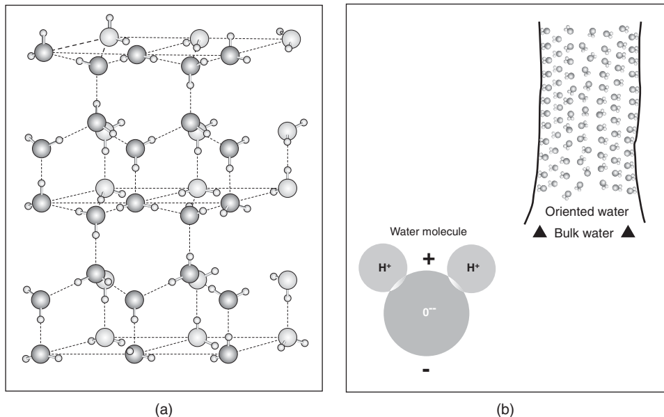
Figure 5-1 (a) Structure of ice. [Reprinted from Pauling, L., The Nature of Chemical Bond , 3d. Cornell University, 1960. Used by permission of the publisher, Cornell University Press]; (b) Structure of oriented water molecules in a micropore. [From Winkler, E.M., Stone: Properties, Durability in Man's Environment , Springer-Verlag, New York, 1973.]
