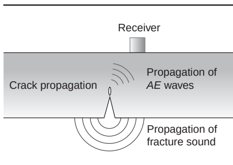
Figure 11-17 Generation, propagation, and detection of acoustic emission (AE). (After Ohtsu, M., The History and Development of Acoustic Emission in Concrete Engineering , Concr. Res. , Vol. 48, pp. 321–330, 1996.)
