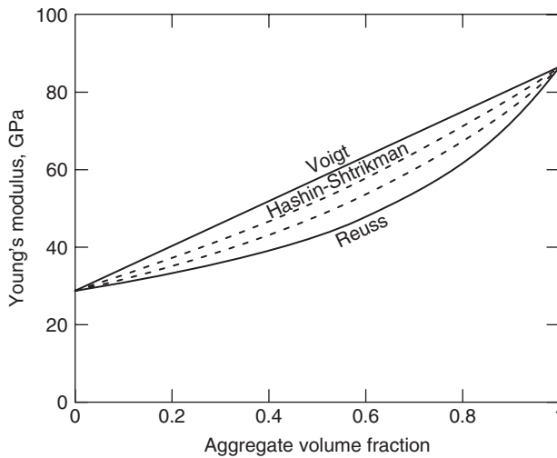
Figure 13-2 Bounds for Young's modulus (elastic moduli of the matrix E_m = 28.7 GPa, K_m = 20.8 GPa and elastic moduli of the aggregate: E_a = 86.7 GPa, K_a = 44 GPa)
