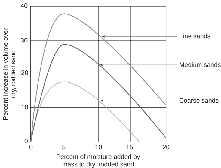
Figure 7-5 (a) Aggregate in various moisture states; (b) bulking due to moisture in fine aggregate. (From Design and Control of Concrete Mixtures , 13th ed., Portland Cement Association, Skokie, IL., pp. 36–37, 1988.)
