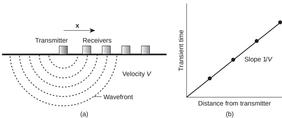
Figure 11-12 (a) Configuration of many receivers using the indirect transmission method and (b) typical plot to determine velocity V using the configuration shown in (a). The material is assumed to be homogeneous and uniform, compare the wave propagation when the material is not uniform, such as shown in Fig 11-13, where a low-velocity layer is on top of a high-velocity material.
