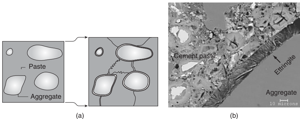
Figure 5-15 (a) Diagrammatic representation of the expansion of a mortar or concrete caused by delayed ettringite formation (DEF). [After Taylor, H.F.W., C. Famy,; K.L. Scrivener, Delayed ettringite formation. Cem. Concr. Res. , Vol. 31, No. 5, pp. 683–693, 2001] (b) Scanning electron micrograph of a mortar affected by DEF. The sample was stored for 4 h at 20°C, heated at 90°C for 12 h and subsequently stored in water for 600 days (micrograph courtesy of C. Famy).
