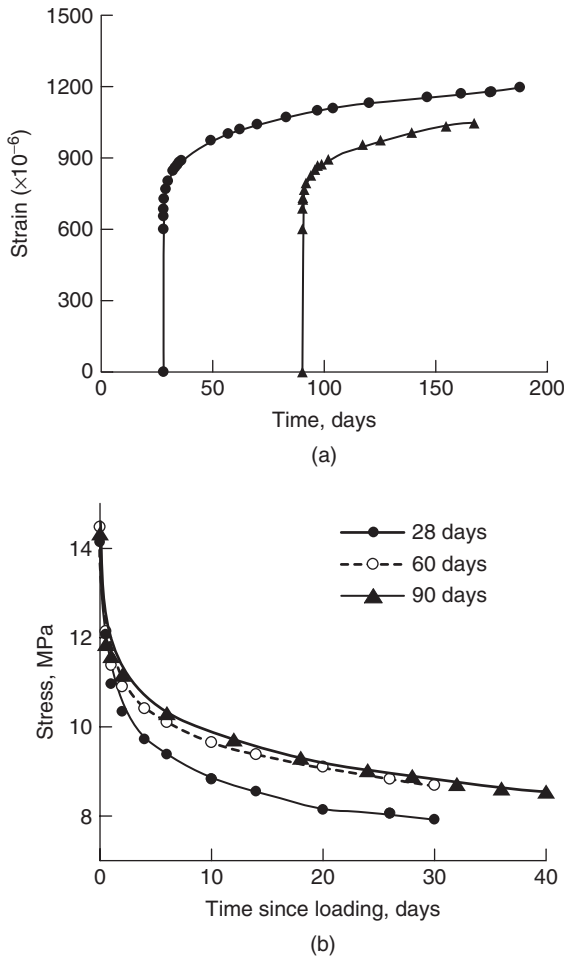
Figure 13-4 (a) Creep test; (b) relaxation test of concrete.
