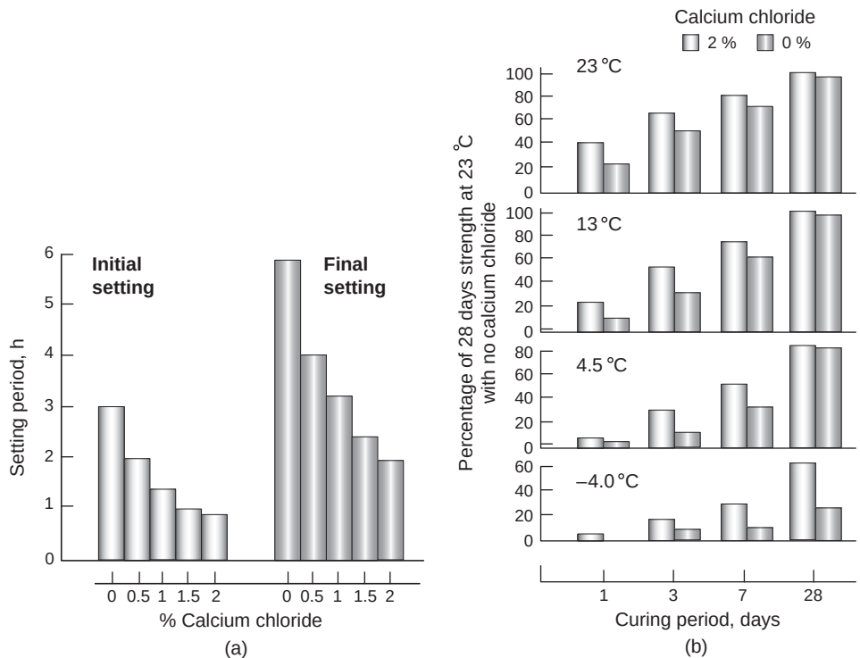
Figure 8-6 Effect of calcium chloride addition on (a) setting time of portland cement (b) effect of calcium chloride addition on strength at various curing temperatures. [From Ramachandran, V.S., Progress in Concrete Technology , Malhotra, V.M., ed., CANMET, Ottawa, pp. 421–450, 1980.]
