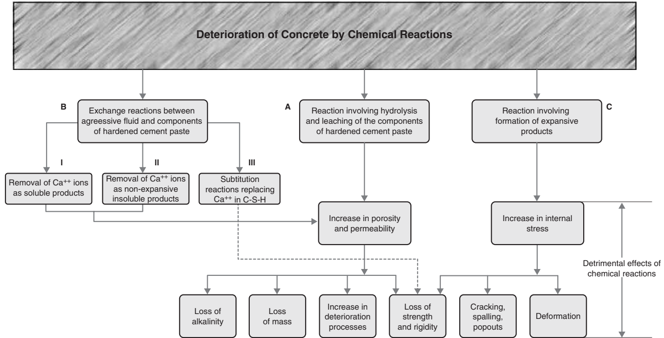
Figure 5-14 Types of chemical reactions responsible for concrete deterioration. A: soft-water attack on calcium hydroxide and C-S-H present in hydrated portland cements; B (I): acidic solution forming soluble calcium compounds such as calcium chloride, calcium sulfate, calcium acetate, or calcium bicarbonate; B (II): solutions of oxalic acid and its salts, forming calcium oxalate; B (III): long-term seawater attack weakening the C-S-H by substitution of \text{Mg}^{2+} for \text{Ca}^{2+} ; C: sulfate attack forming ettringite and gypsum, alkali-aggregate attack, corrosion of steel in concrete, hydration of crystalline \text{MgO} and \text{CaO} . (From Mehta, P.K., and B.C. Gerwick, Jr., Concr. Int. , Vol. 4, pp. 45–51, 1982.)
