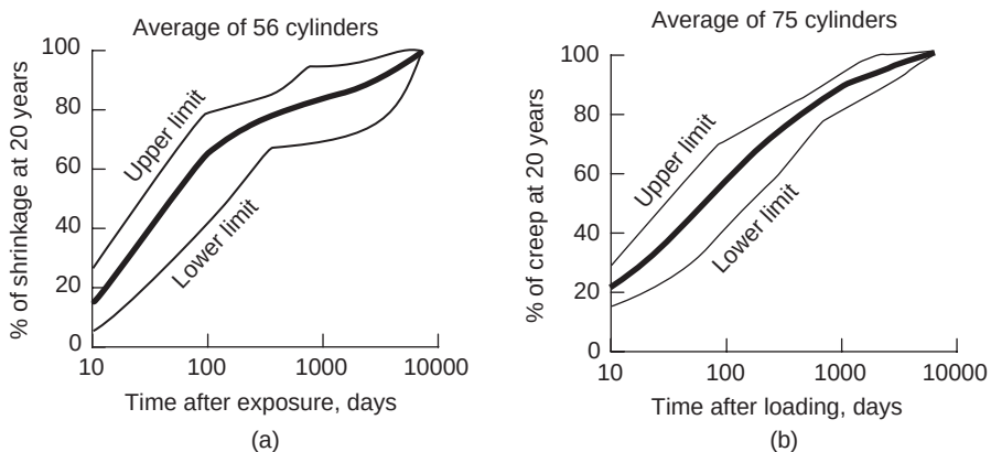
Figure 4-12 The time dependency of (a) drying shrinkage and (b) creep. (From Troxell, G.E. et al., Proc. ASTM , Vol. 58, 1958. Reprinted with permission from ASTM. Copyright ASTM, 1916 Race Street, Philadelphia, PA.)
