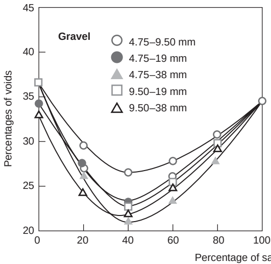
Figure 7-6 Reduction in the volume of voids on mixing fine and coarse aggregates. [(a), From Design and Control of Concrete Mixtures , 13th ed., Portland Cement Association, Skokie, IL, p. 33, 1988; (b) From Walker, S., Circular 8 , National Sand and Gravel Association, 1930.]
