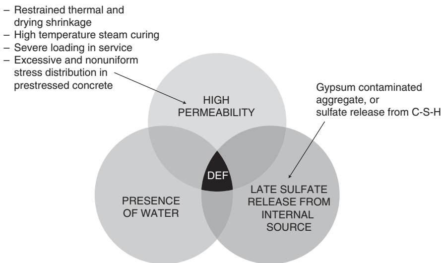
Figure 5-16 Holistic approach for expansion and cracking by delayed ettringite formation.
