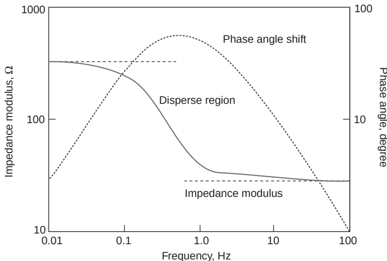
Figure 11-31 A plot of impedance spectrum plot with frequency for the equivalent circuit described in Fig. 11-29 using the following values: R_c = 30 \, \Omega , R_p = 300 \, \Omega , and C_{dl} = 0.003 \, \text{F} .
