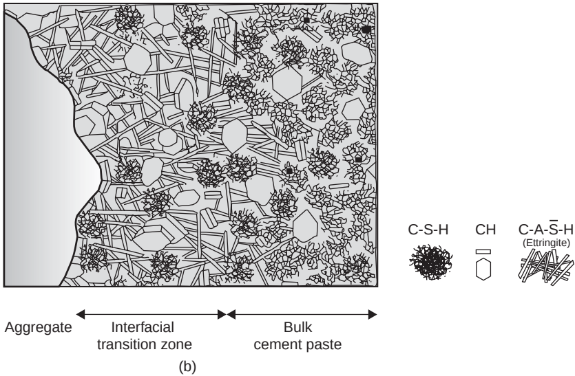
Figure 2-14 (a) Scanning electron micrograph of the calcium hydroxide crystals in the interfacial transition zone. (b) Diagrammatic representation of the interfacial transition zone and bulk cement paste in concrete.
