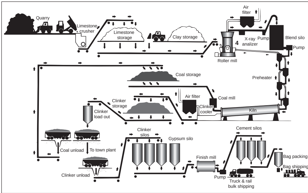
Figure 6-2 Flow diagram of the dry process for portland cement manufacture.
