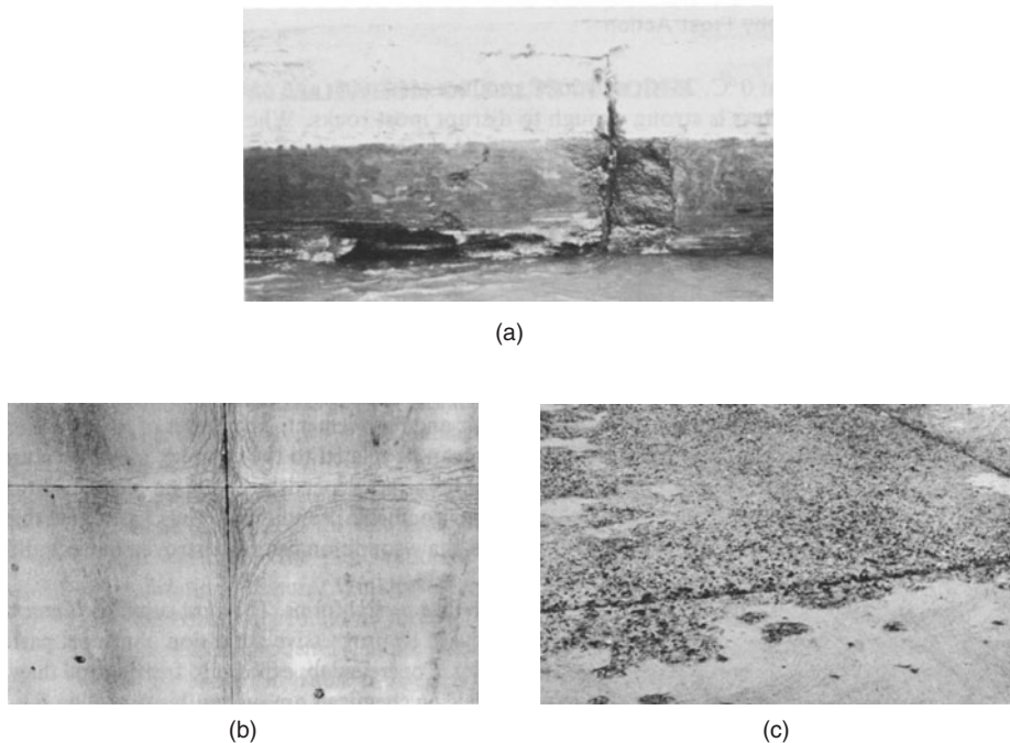
Figure 5-6 Types of frost action damage in concrete: (a) deterioration of a non-air-entrained concrete-retaining wall along the saturation line (Lock and Dam No. 3, Monongahela River, Pittsburg, PA); (b) severe D-cracking along longitudinal and transverse joints of a 9-year-old pavement; (c) scaling of a concrete surface. [(a) Photograph courtesy of J.M Scanlon, U.S. Army Corps of Engineers, Vicksburg, MS); (b) photograph courtesy of D. Stark, from Report RD 023.01P , Portland Cement Association, Skokie, IL.,1974; (c) photograph courtesy of R.C. Meininger, from Concrete in Practice , Publ. 2, National Ready Mixed Concrete Association, Silver Springs, MD.]
