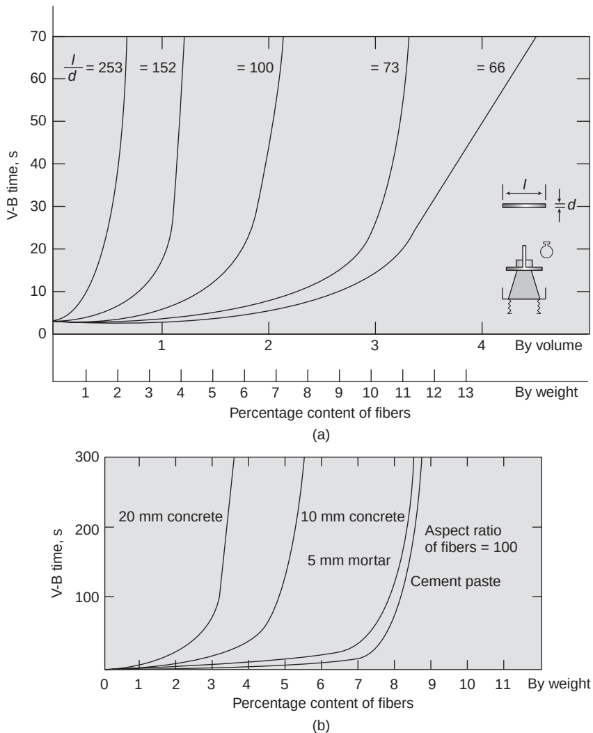
Figure 12-17 (a) Effect of fiber aspect ratio on workability of mortar; (b) effect of aggregate size and fiber content on workability. (From Edington, J., D.J. Hannant, and R.I.T. Williams, BRE Current Paper 69/74, July 1974. By courtesy of Building Research Establishment, U.K., and reproduced by permission of Her Majesty's Stationery Office.)
