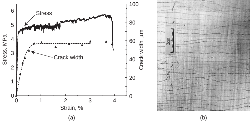
Figure 12-23 (a) Tensile stress-strain and crack-width-strain relations for a pseudo strain-hardening ECC; (b) controlled damage of engineered cementitious composite. (Courtesy of V. Li.)
