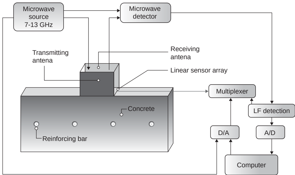
Figure 11-42 Block diagram of the microwave camera.
