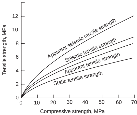
Figure 3-18 Design chart for tensile strength. (From Raphael, J., J. ACI, Proc. , Vol. 81, No. 2, pp. 158–164, 1984.)
