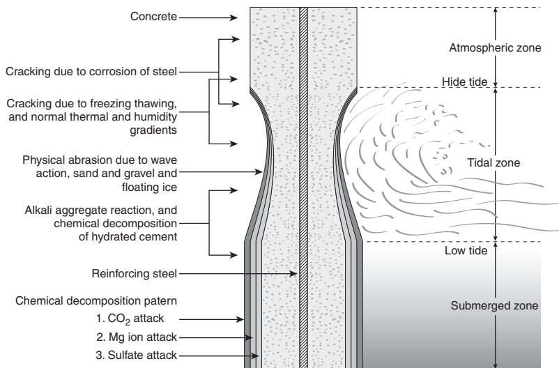
Figure 5-28 Diagrammatic representation of a reinforced concrete cylinder exposed to seawater. (From Mehta, P.K., Performance of Concrete in Marine Environment , ACI SP- 65, pp. 1–20, 1980.)
