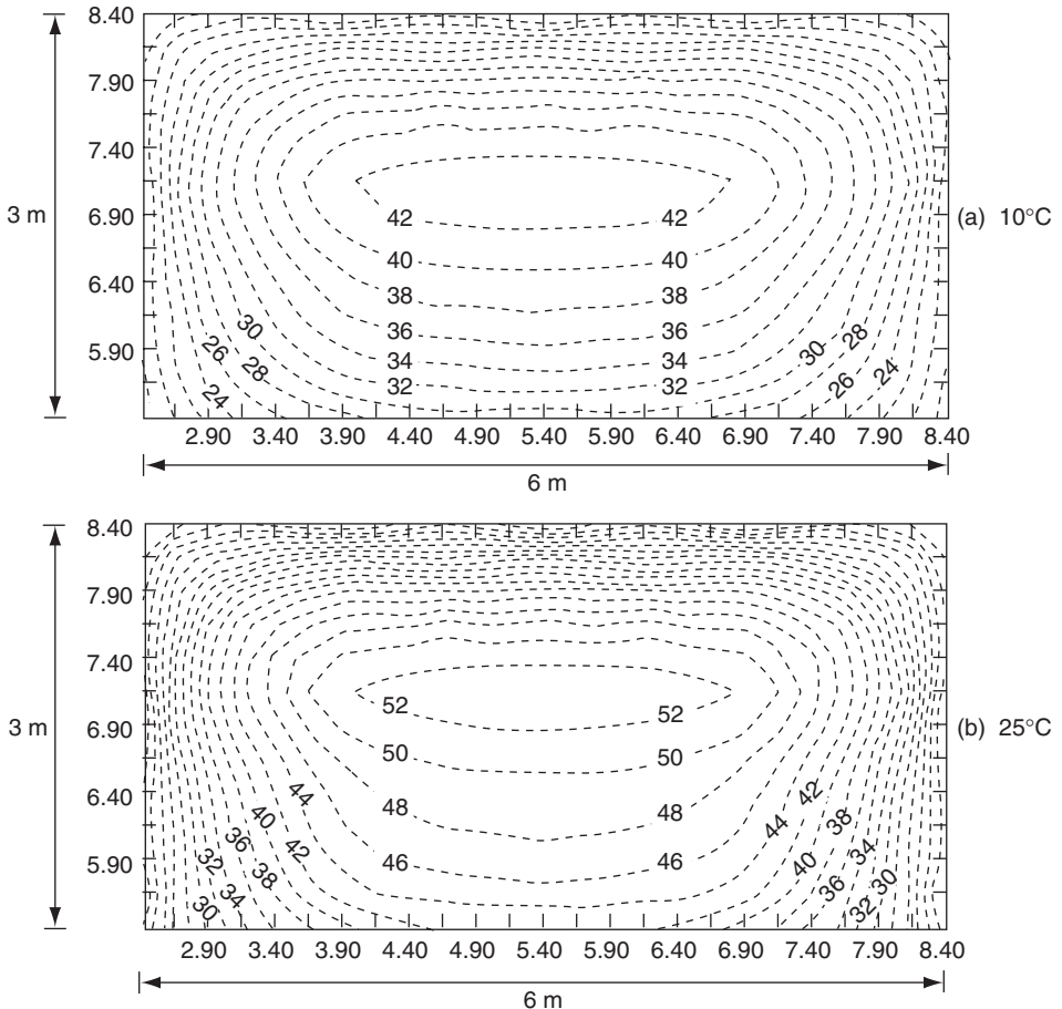
Figure 13-20 Effect of fresh concrete on the maximum temperature distribution.
