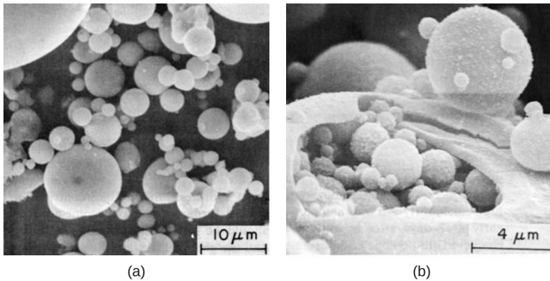
Figure 8-9 Scanning electrons micrographs of a typical Class F fly ash: (a) spherical glassy particles; (b) a plerosphere.
