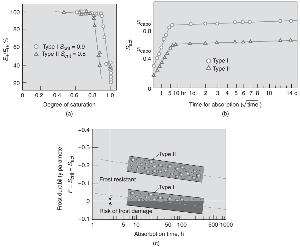
Figure 5-11 Method of predicting the frost resistance of concrete. (From Betong-handboken , Svensk Byggtjänst, Stockholm, 430–433, 1980.)
