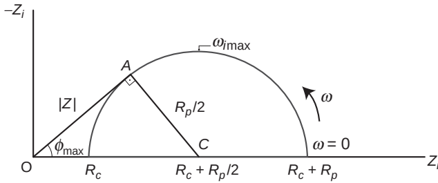
Figure 11-30 Nyquist plot for the impedance of the electric circuit shown in Fig. 11-29.
