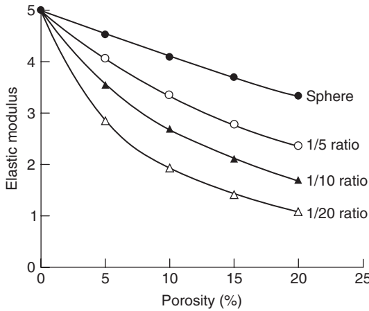
Figure 13-3 Effect of porosity and shape of pores on the elastic modulus of a material.
