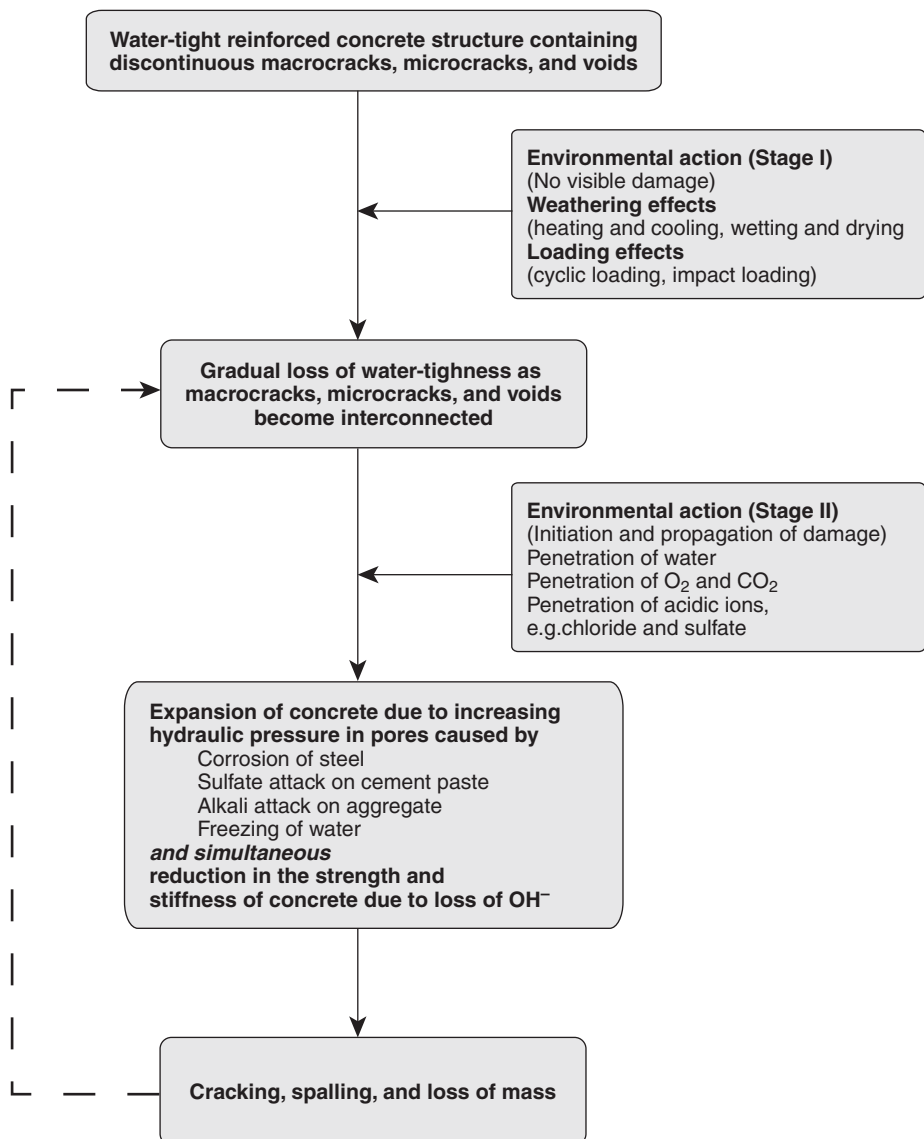
Figure 5-26 A holistic model of deterioration of concrete from commonly encountered environmental effects (Mehta, P.K., ACI, SP-144 , pp. 1–34, 1994; Concr. Int. , Vol. 19, No. 7, pp. 69–76, 1997.).
