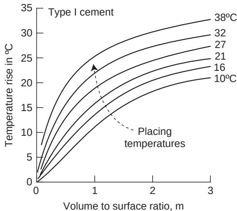
Figure 4-22 Temperature rise of concrete members containing 223 kg/m 3 of cement. (ACI Committee 207. Effect of restraint, volume changes, and reinforcement on cracking of massive concrete, 1995.)
