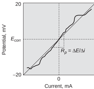
Figure 11-26 A representation of the polarization resistance curve.
