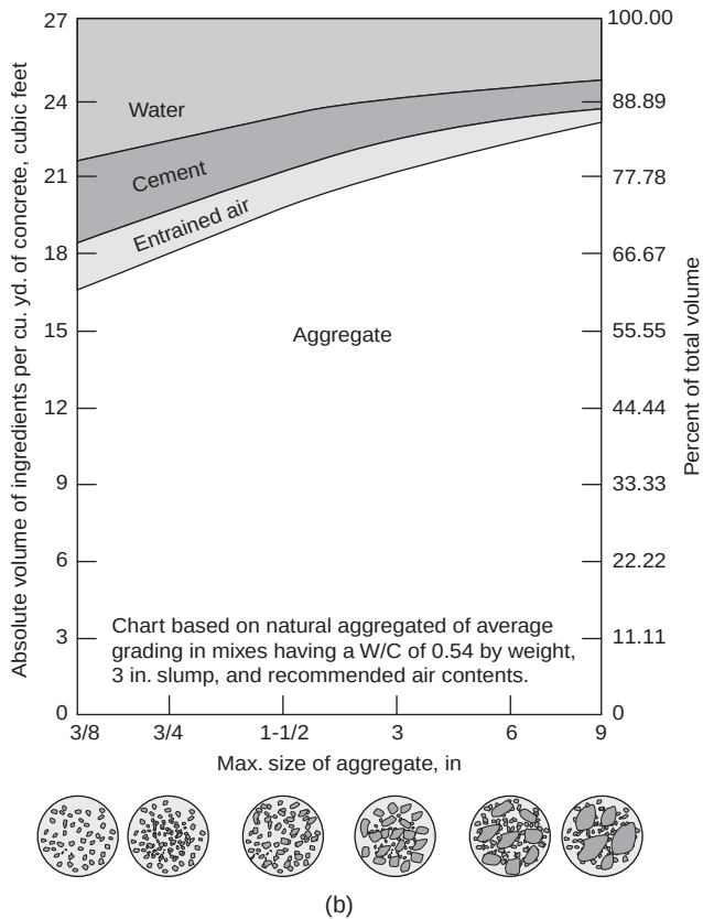
Figure 12-25 Effect of maximum size of aggregate on (a) water content of concrete, (b) concrete mix proportions. (From Concrete Manual , 8th ed., U.S. Bureau of Reclamation, Denver, Colorado, 1981.)
