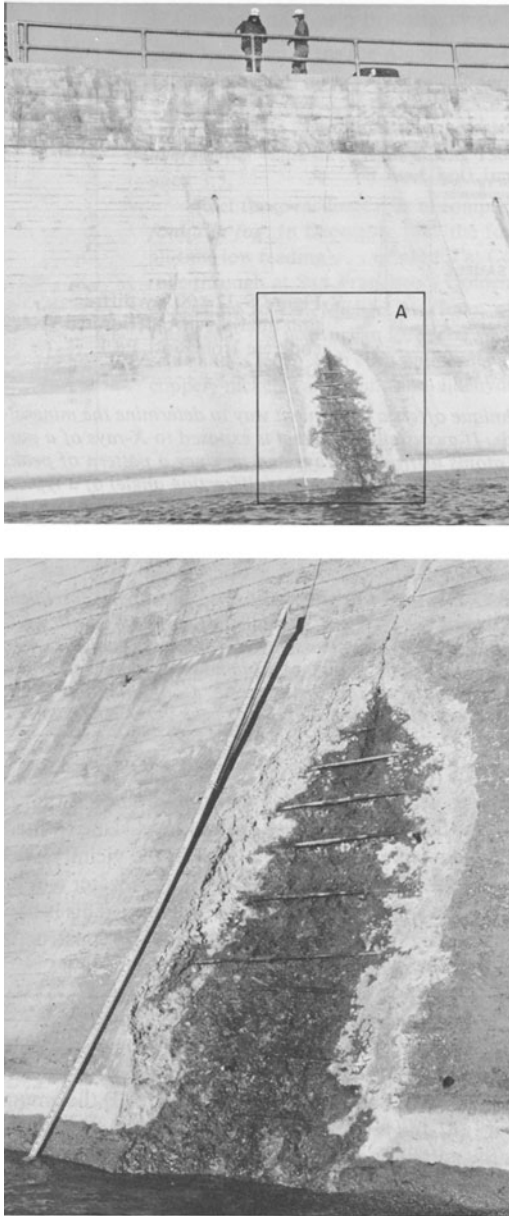
Figure 5-17 Sulfate attack on concrete in Fort Peck Dam, 1971. (Photographs courtesy of T.J. Reading, formerly Materials Engineer of the Missouri River Division, U.S. Corps of Engineers.)
