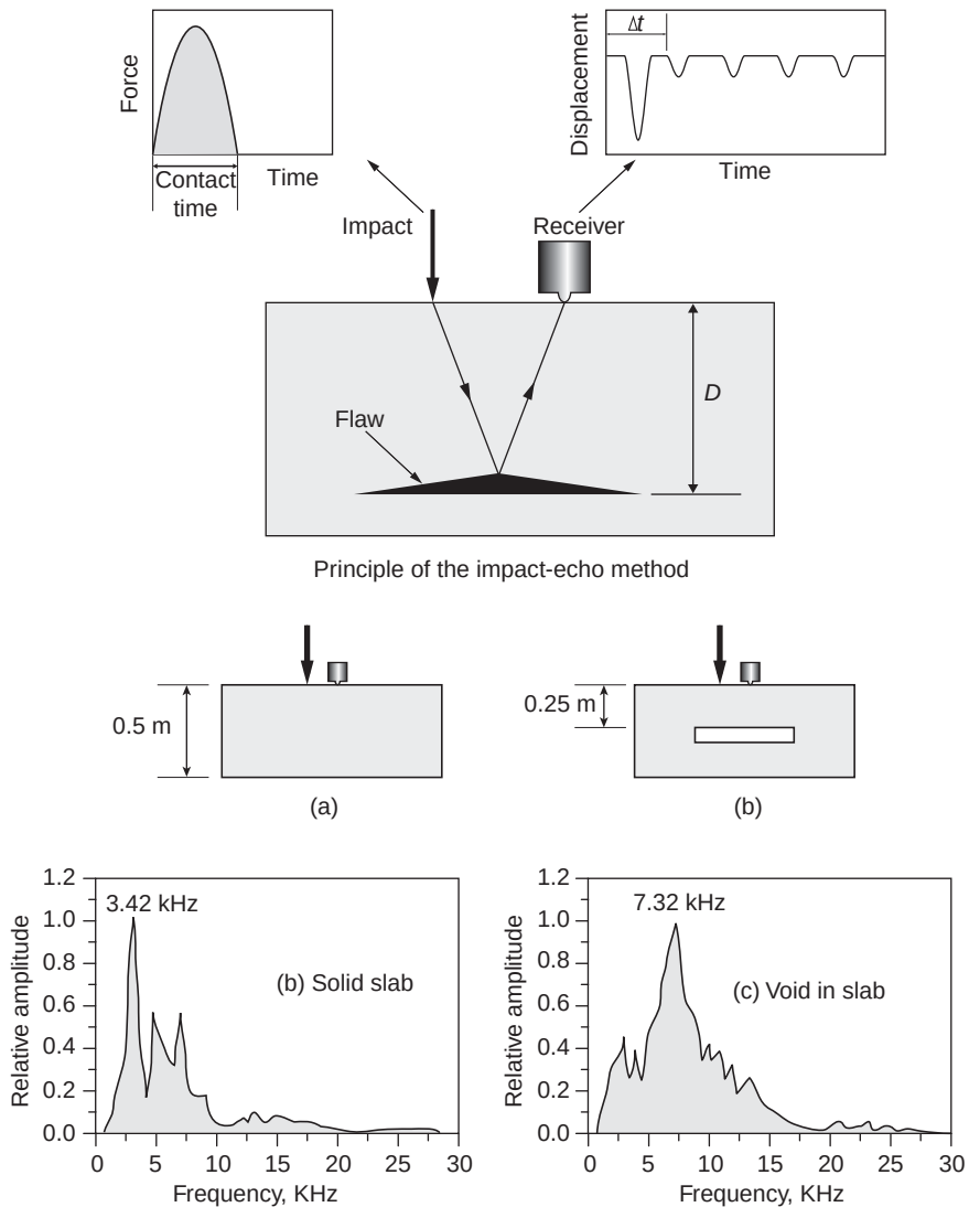
Figure 11-15 Application of the impact-echo method to identify a disk-shaped void in a slab (After ACI 228.2R-98, Nondestructive Test Methods for Evaluation of Concrete Structures ).
