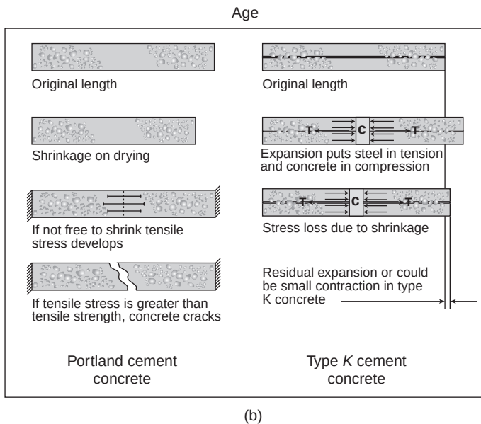
Figure 12-10 (a) Comparison of length change characteristics between portland cement and Type K cement concrete; (b) illustration showing why Type K cement concrete is resistant to cracking from drying shrinkage. (From Williams, J.V., Jr., Concr. Int. , Vol. 3, No. 4, p. 58, 1981.)
