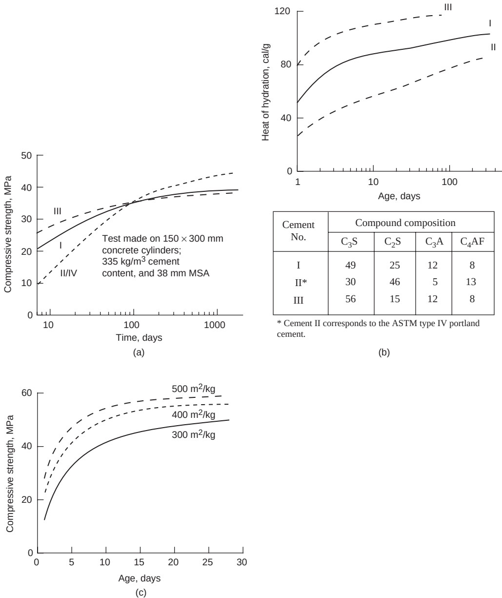
Figure 6-11 (a) Influence of cement composition on strength; (b) influence of cement composition on heat of hydration; (c) influence of cement fineness on strength. [Data for (a) and (b) are adapted from Concrete Manual , U.S. Bureau of Reclamation, 1975, pp. 45–46; data for (c) is taken from Beton-Bogen , Aalborg Cement Company, Aalborg, Denmark, 1979.]
