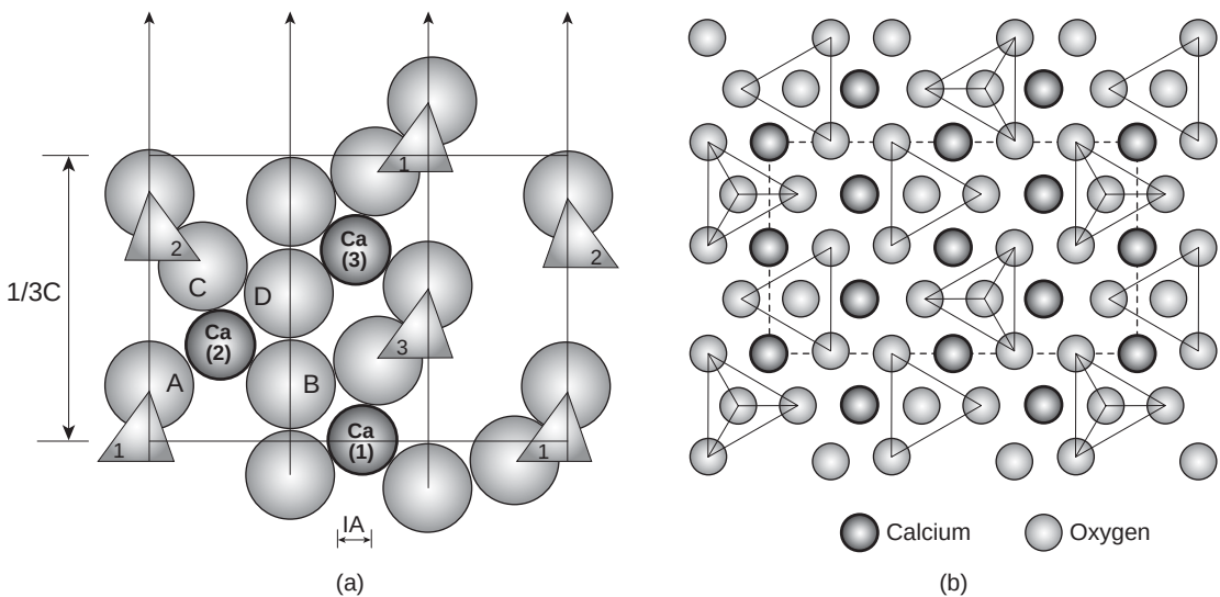
Figure 6-5 Crystal structures of (a) 3\text{CaO-SiO}_2 (b) \gamma\text{-}2\text{CaO-SiO}_2 . Part (a) shows a vertical section of the bottom layer of the pseudo structure of 3\text{CaO-SiO}_2 through the long diagonal of the cell. Only the oxygen atoms in the symmetry plane are shown as plain circles. 1, 2, and 3 are sections of \text{SiO}_4 tetrahedron. Calcium atoms are labeled. In (b), silicon atoms are not shown; they occur at the center of the silica tetrahedra. [Lea, F.M., The Chemistry of Cement and Concrete , Chemical Publishing Company, New York, 1971, by permission of Edward Arnold (Publishers)]
