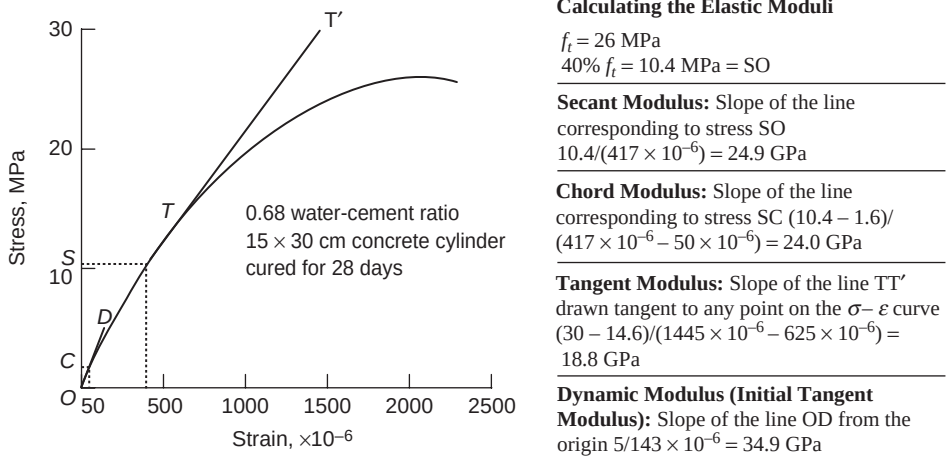
Figure 4-4 Different types of elastic moduli and the method by which these are determined.
