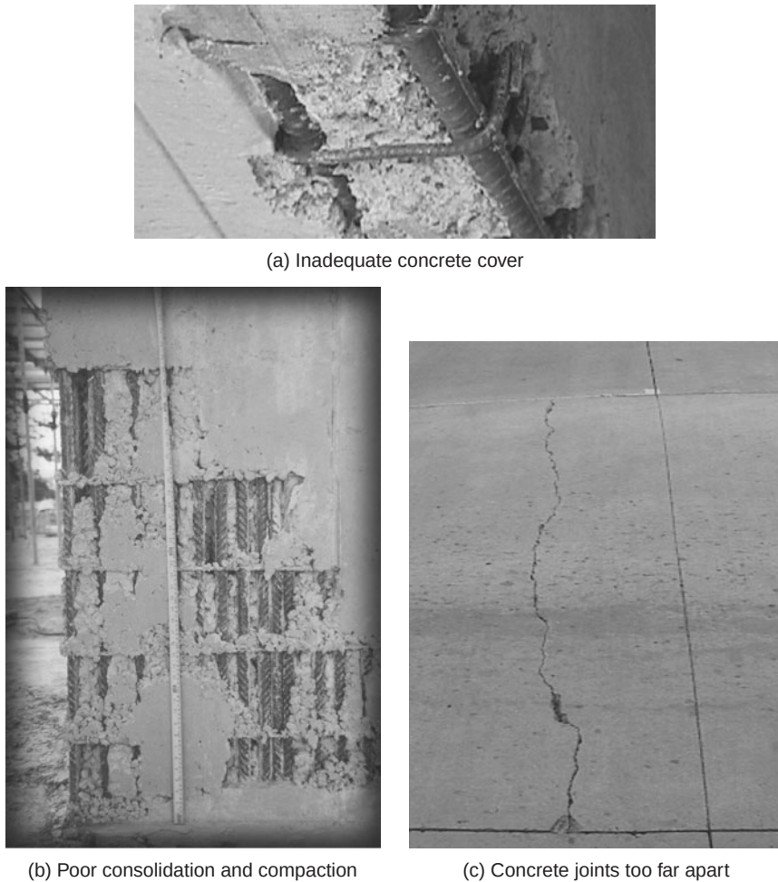
Figure 10-17 Typical concrete damage caused by improper construction practice. [Photos courtesy from Carlos Videla ( a and c ) and Paulo Barbosa ( b )]
