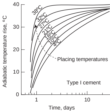
Figure 4-21 Effect of placing temperature on temperature rise of mass concrete containing 223 kg/m 3 on Type I cement. (ACI Committee 207. Effect of restraint, volume changes, and reinforcement on cracking of massive concrete, 1995.)
