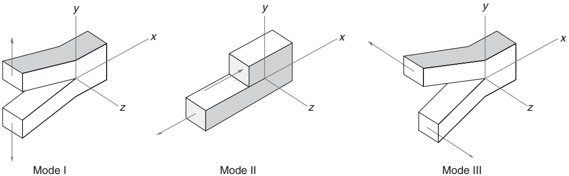
Figure 13-25 Basic modes of loading. (After Hertzberg, R.W., Deformations and Fracture Mechanics of Engineering Materials , Wiley, New York, p. 262, 1976.)
