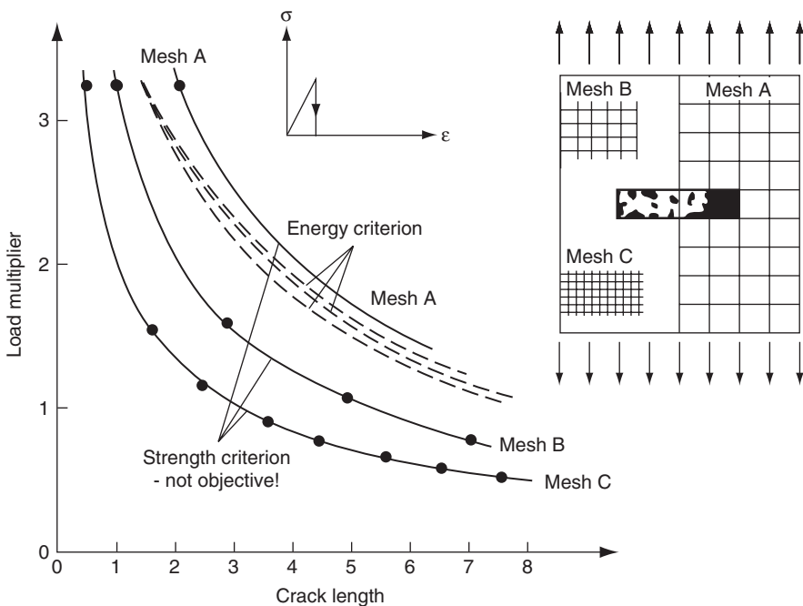
Figure 13-22 Example of mesh sensitivity. (From Bazant, Z.P., and L. Cedolin, Stability of Structures , Oxford University Press, New York, p. 917, 1991.)
