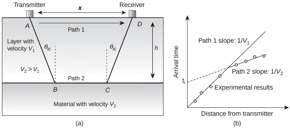
Figure 11-13 Effect of a low-velocity layer on the wave propagation. (a) geometric construction for determination of the thickness h , (b) graphical procedure to determine the value of t_i and consequently the thickness h . See Eq. (11-19).
