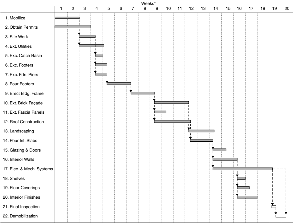
Figure 8.13 Expanded bar-net schedule for the small gas station.
