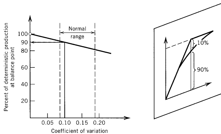
Figure 14.15 Plot of cycle time coefficient of variation.
