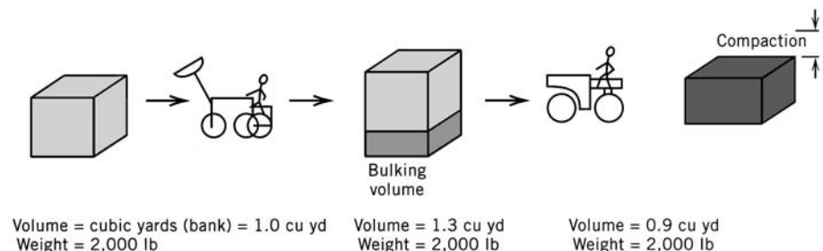
Figure 14.1 Volume relationships.
