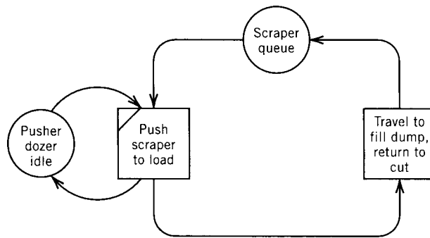
Figure 14.9 Scraper-pusher dual-cycle model.
