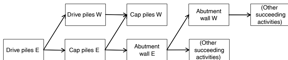
Figure 8.12 Segment of precedence diagram for small bridge.
