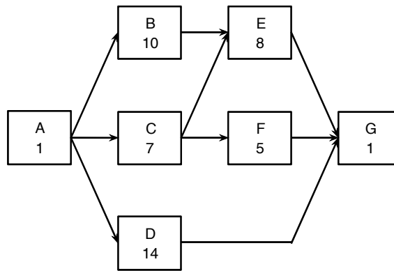
Figure 8.18 Example Diagram with traditional relationships.
