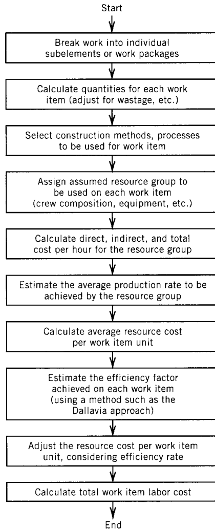
Figure 16.9 Resource enumeration method of estimating.
