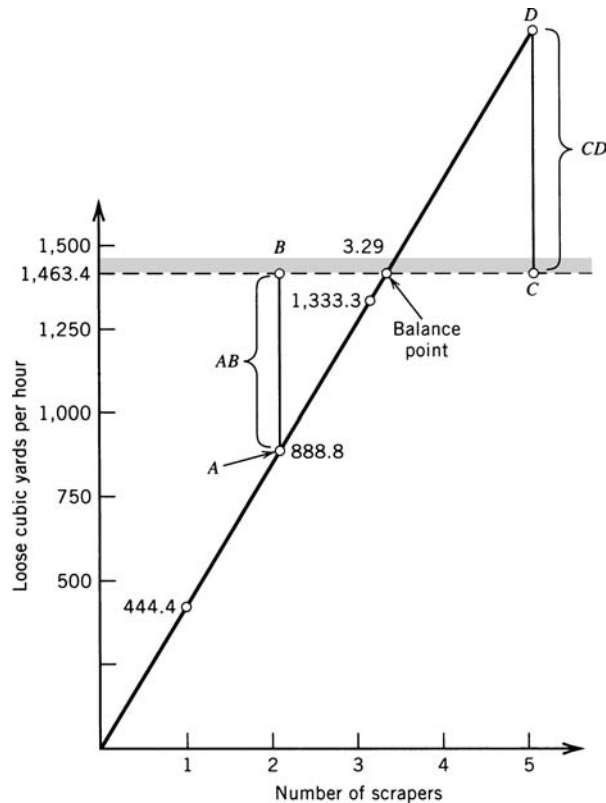
Figure 14.12 Productivity plot.
