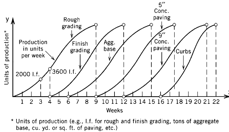
Figure 9.7 Velocity diagrams for a road construction project.
