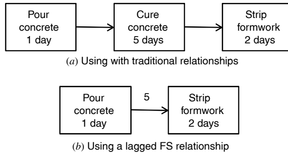
Figure 8.14 Modeling the sequence of concrete pour-cure-stripping.
