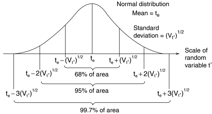
Figure 9.1 Selected areas under the normal distribution curve.
