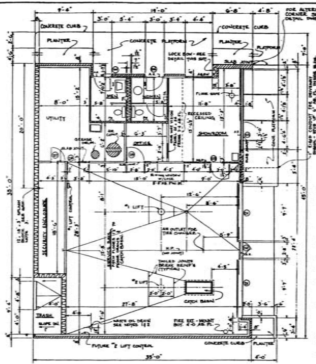
FLOOR PLAN
