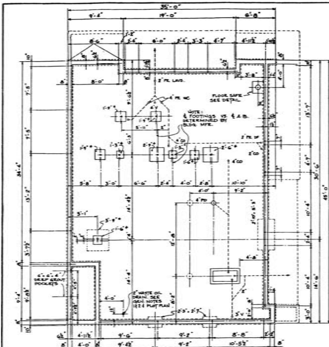
FOUNDATION & ANCHOR BOLT PLAN
