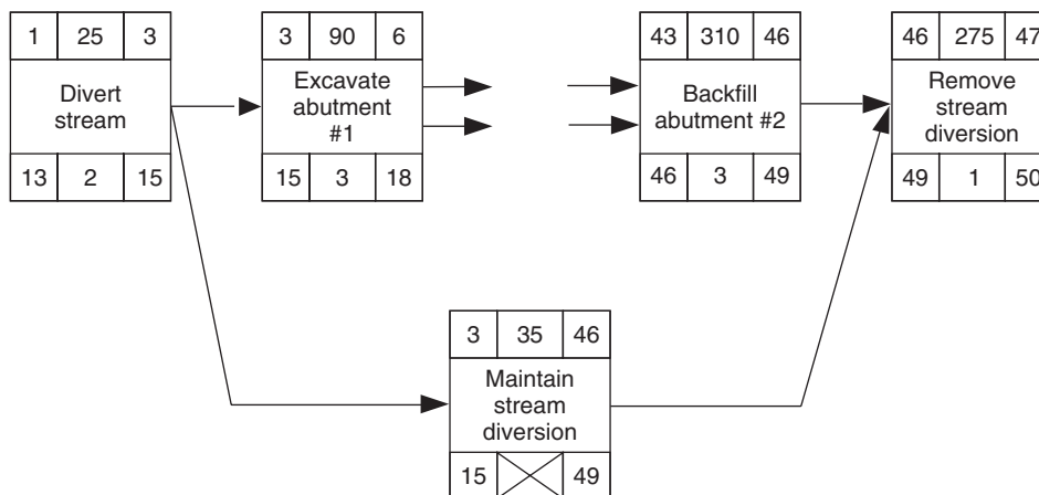
Figure 5.13 Highway bridge, hammock activity
