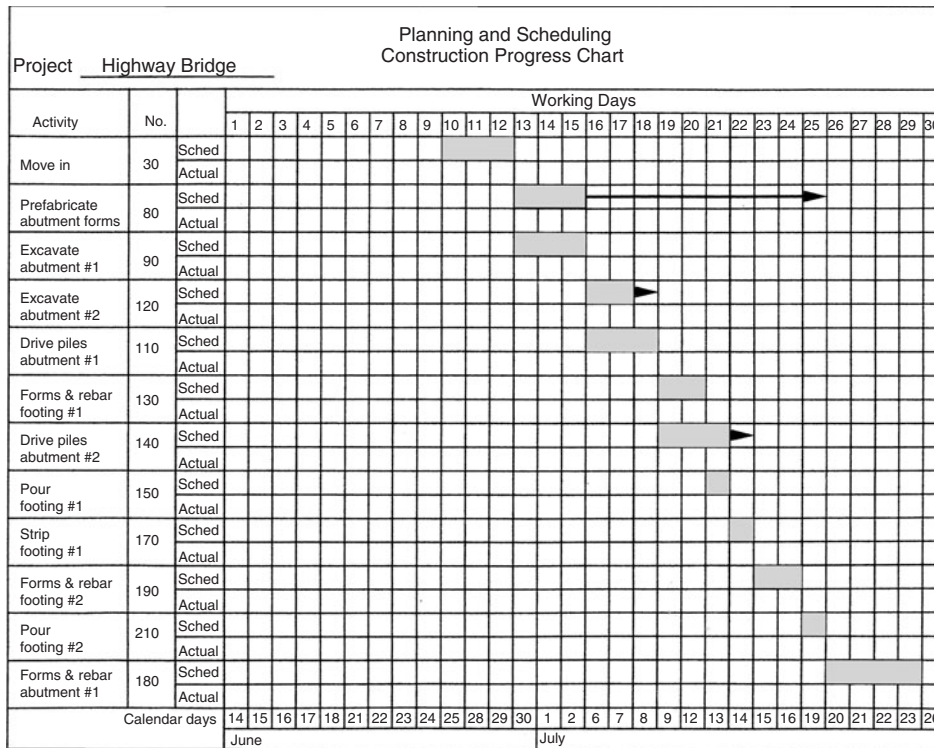
Figure G.1 Original work schedule
