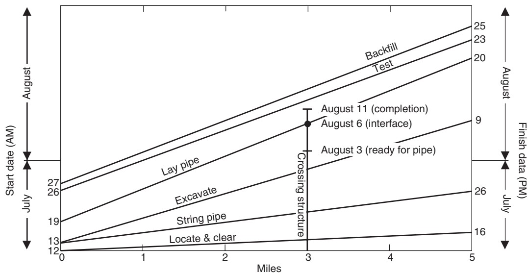
Figure 5.16 Pipeline relocation, bar chart schedule
