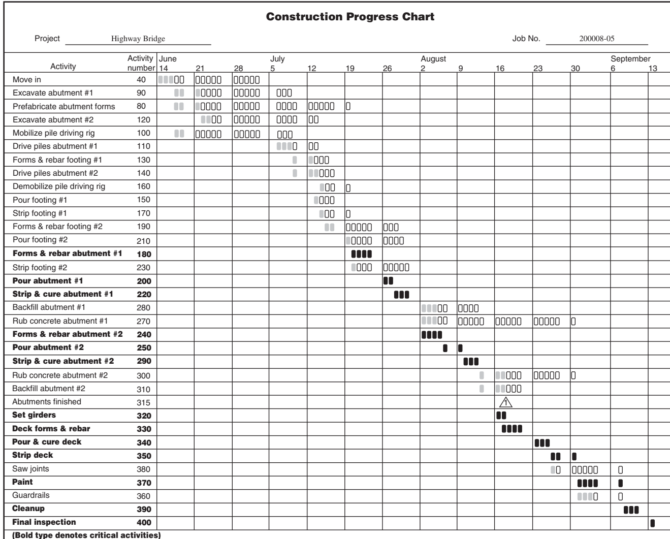
Figure 5.15 Highway bridge, bar chart schedule
