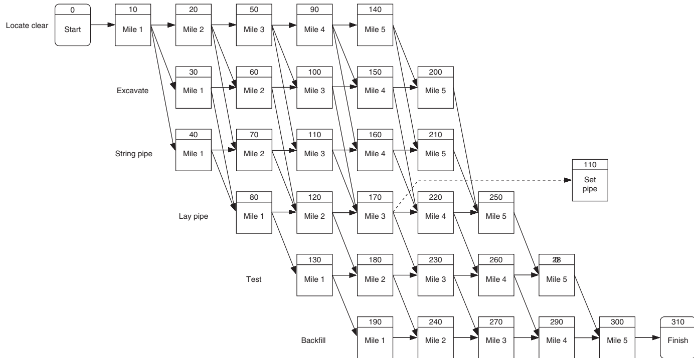
Figure 4.5 Pipeline relocation, precedence diagram planning
