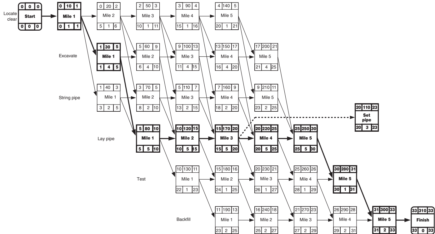
Figure 5.10 Pipeline relocation, precedence diagram time computations
