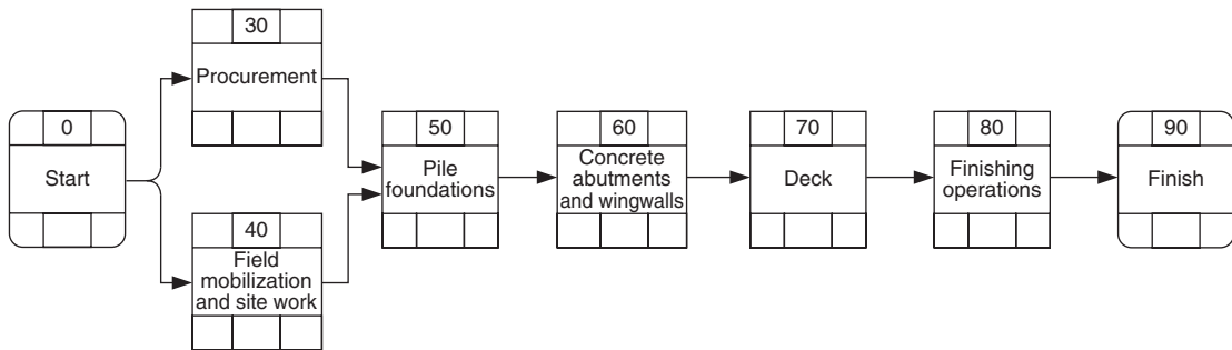
Figure 4.2 Highway bridge, general job plan
