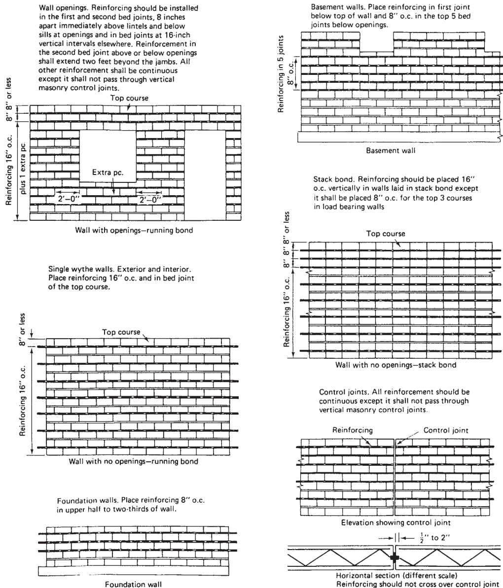
FIGURE 11.16. Reinforcement Layout.
