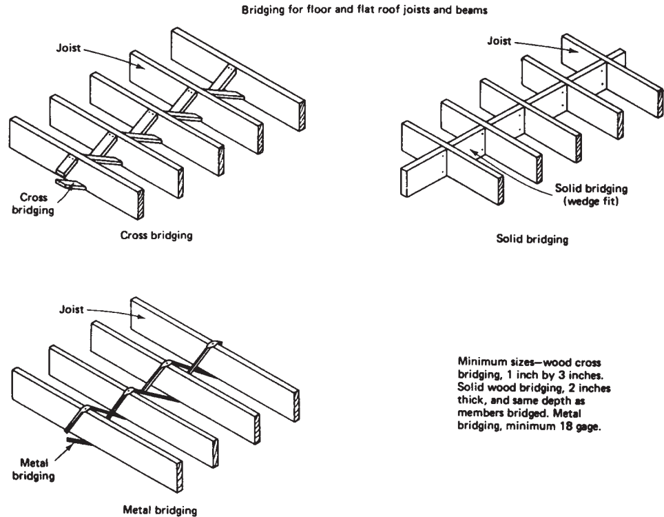
FIGURE 13.20. Bridging.
