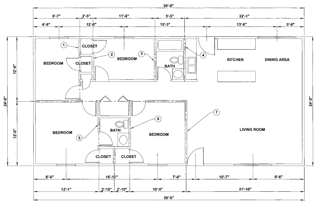
FIGURE 13.8. Floor Plan.
