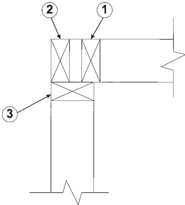
FIGURE 13.25. Corner Stud.
