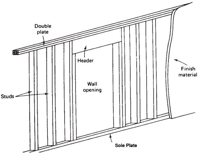
FIGURE 13.23. Wall Framing.
