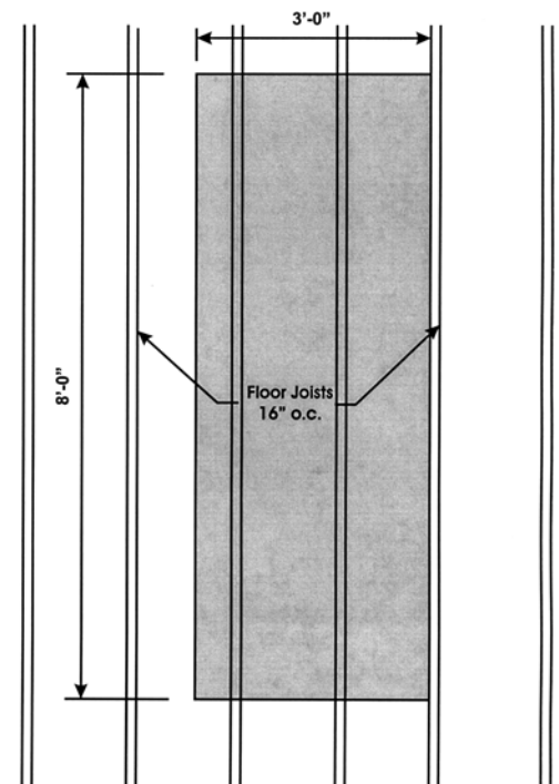
FIGURE 13.17. Joist Openings.
