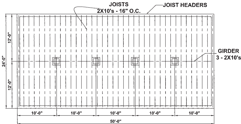
FIGURE 13.5. Floor Framing Plan.
