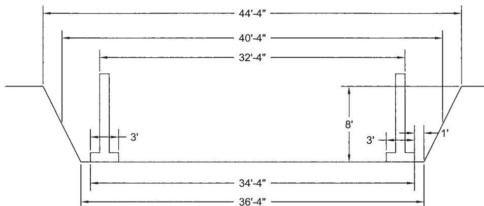
FIGURE 9.34. Basement Cross-Section.
