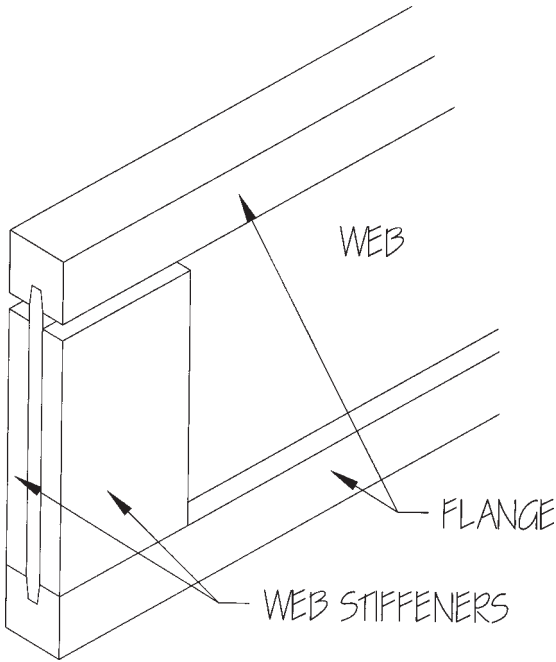
FIGURE 13.6. Wood I-Joist.
