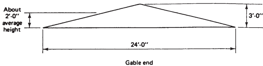
FIGURE 13.35. Gable Average Height.
