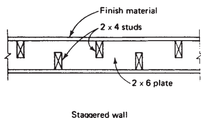
FIGURE 13.43. Special Wall Construction.
