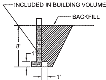
FIGURE 9.39. Footing Backfill.
