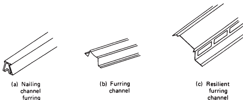
FIGURE 16.2. Metal Furring.
