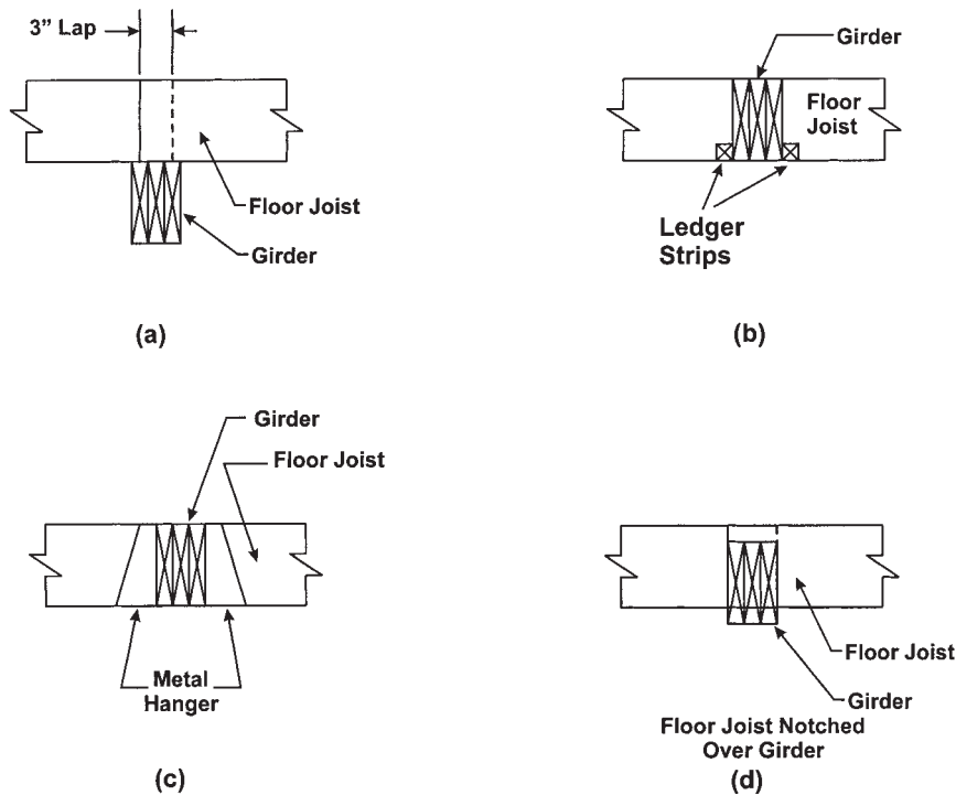
FIGURE 13.11. Joist/Girder Details.
