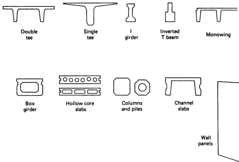
FIGURE 10.34. Precast Shapes.
