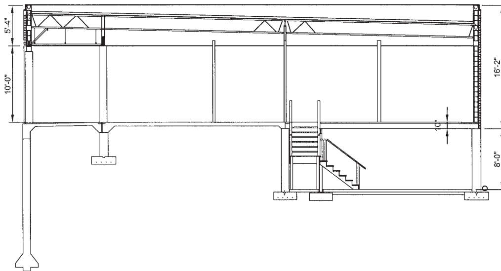
FIGURE 11.9. Wall Section.
