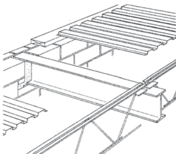
Steel Joists, Beams and Deck on Bearing Walls
