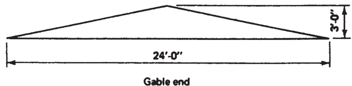
FIGURE 13.34. Gable End Sketch.
