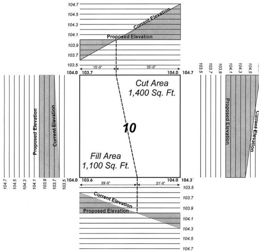
FIGURE 9.12. Grid 10 Layout.
