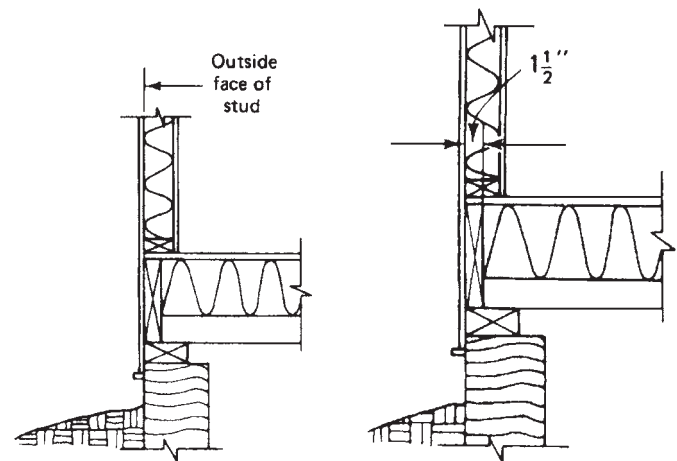
FIGURE 13.9. Joist Headers.
