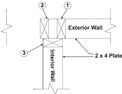
FIGURE 13.27. Wall Intersection Detail (2 × 4s).
