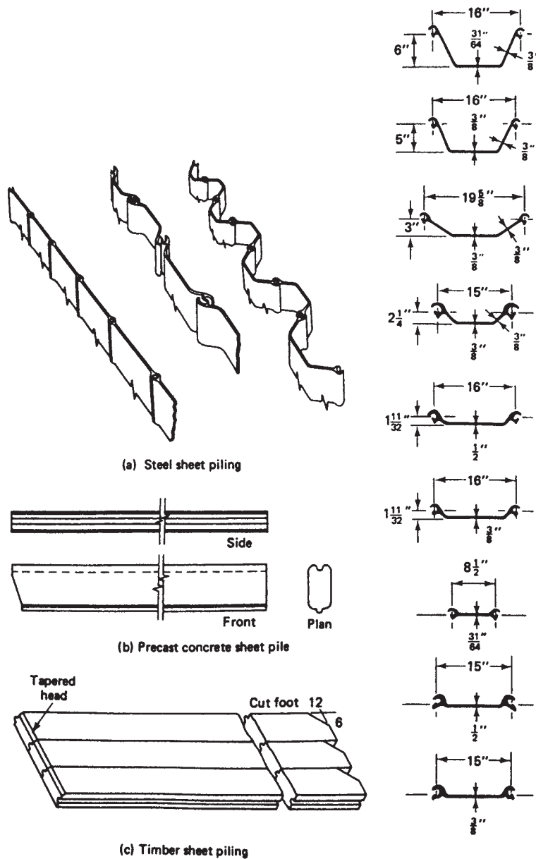
FIGURE 9.30. Sheet Piling.
