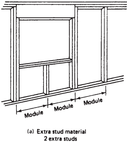
FIGURE 13.32. Wall Openings.
