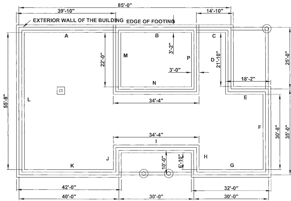
FIGURE 14.5. Foundation Walls.
