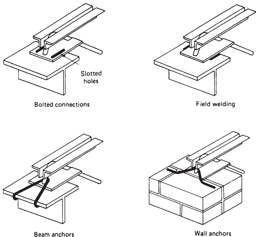
FIGURE 12.8. End Anchorage.
