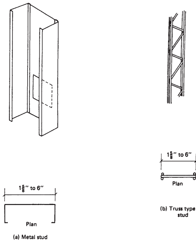
FIGURE 16.1. Metal Studs.
