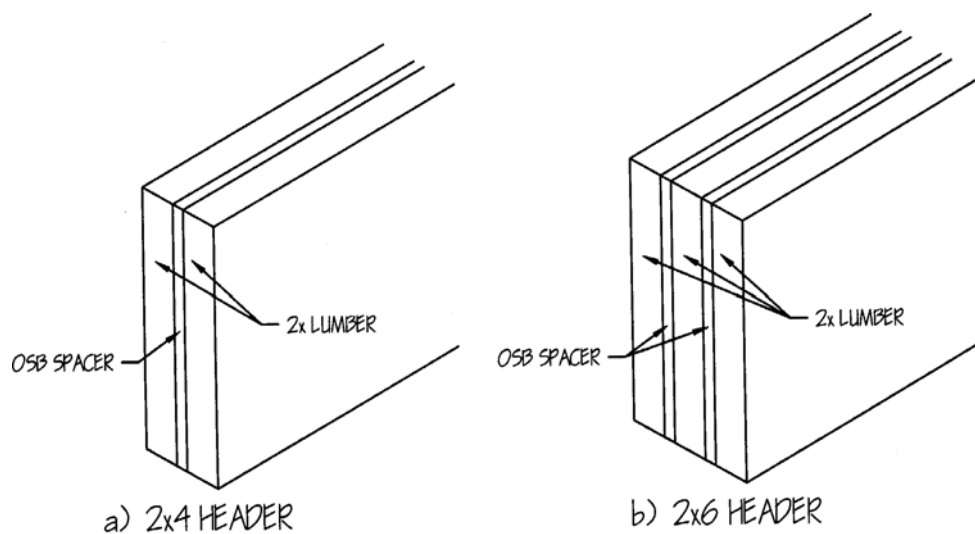
FIGURE 13.37. 2 × Header Construction.
