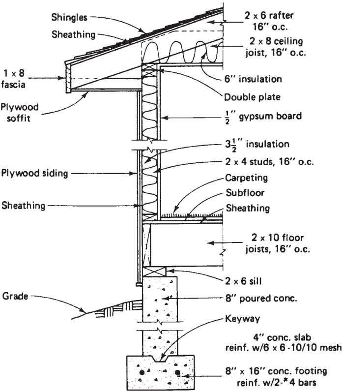
FIGURE 13.39. Typical Wall Section.
