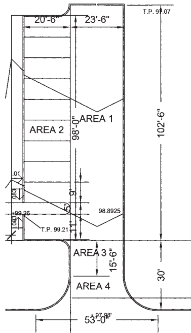
FIGURE 9.45. Parking Lot.
