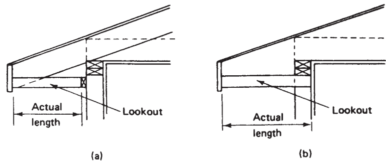
FIGURE 13.52. Lookouts.
