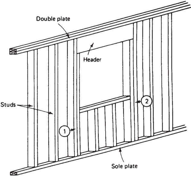
FIGURE 13.30. Wall Opening.
