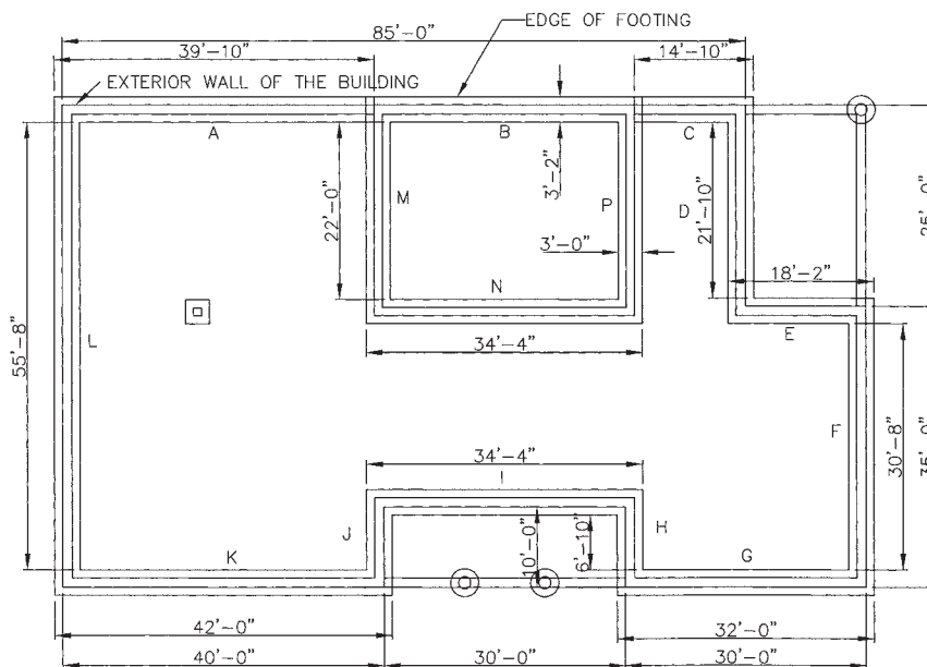
FIGURE 10.1. Foundation Layout.
