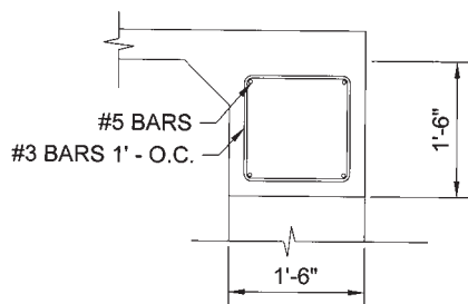
FIGURE 10.24. Grade Beam Details.
