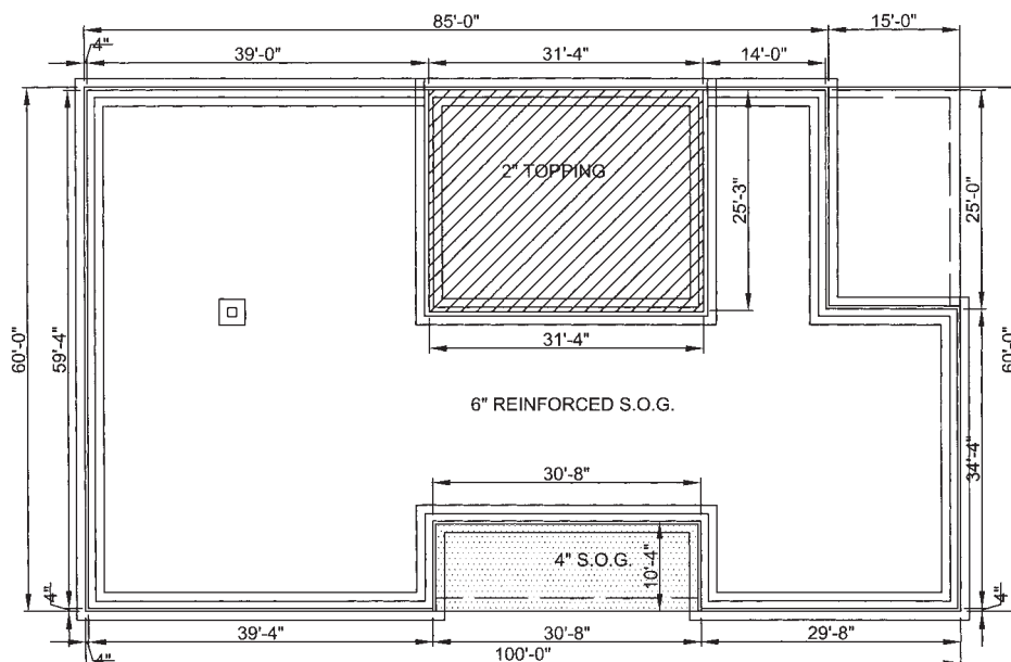
FIGURE 10.15. Slab Area.
