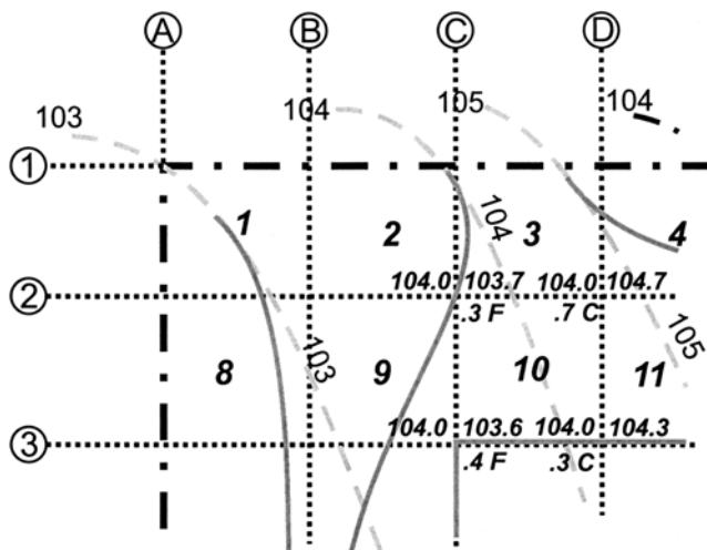
FIGURE 9.11. Grid 10.
