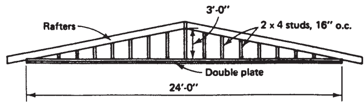
FIGURE 13.33. Gable End Frame.
