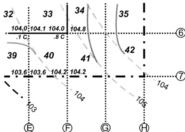
FIGURE 9.10. Excerpt of Grid 40.
