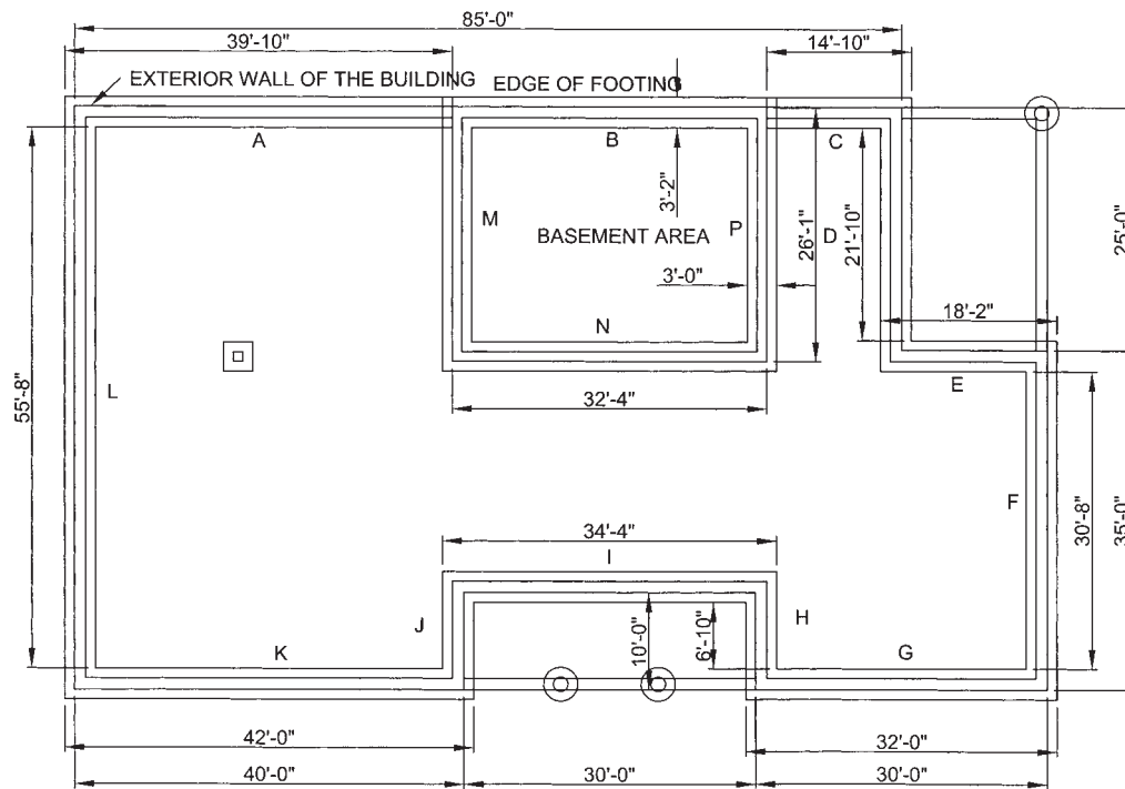
FIGURE 9.32. Building Plan.
