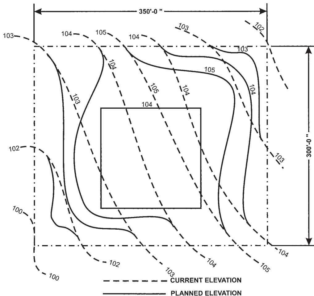
FIGURE 9.3. Sample Site Plan.
