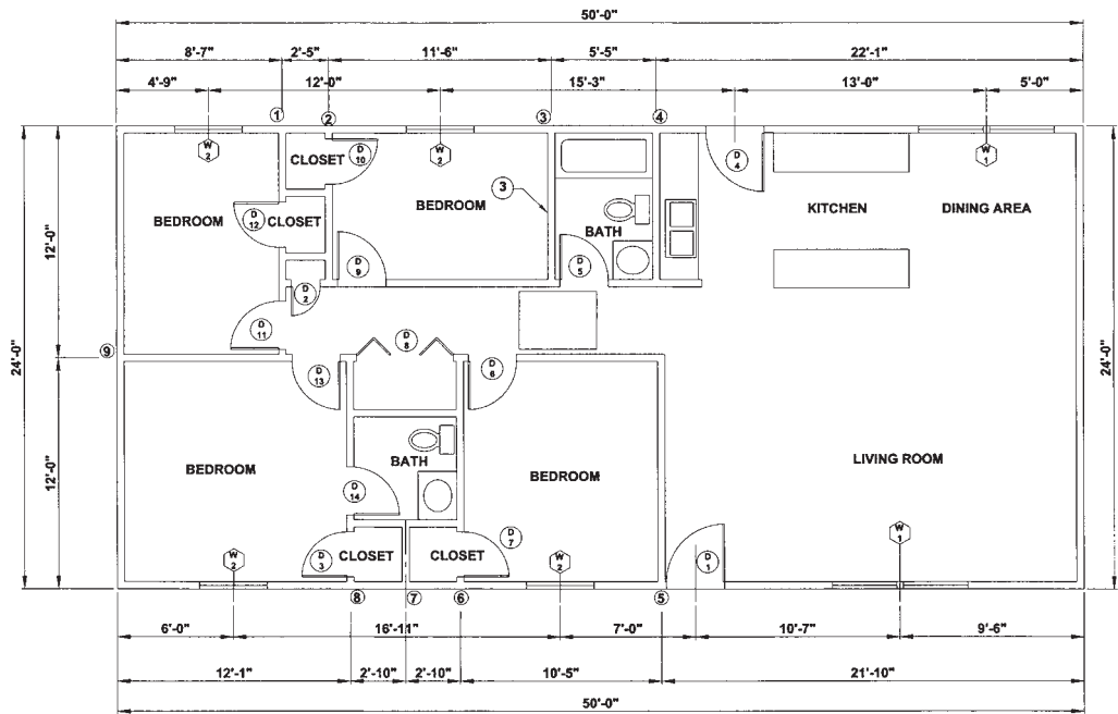
FIGURE 13.28. Floor Plan.
