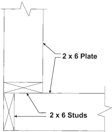
Exterior Corner
