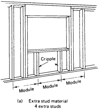
FIGURE 13.31. Wall Openings.
