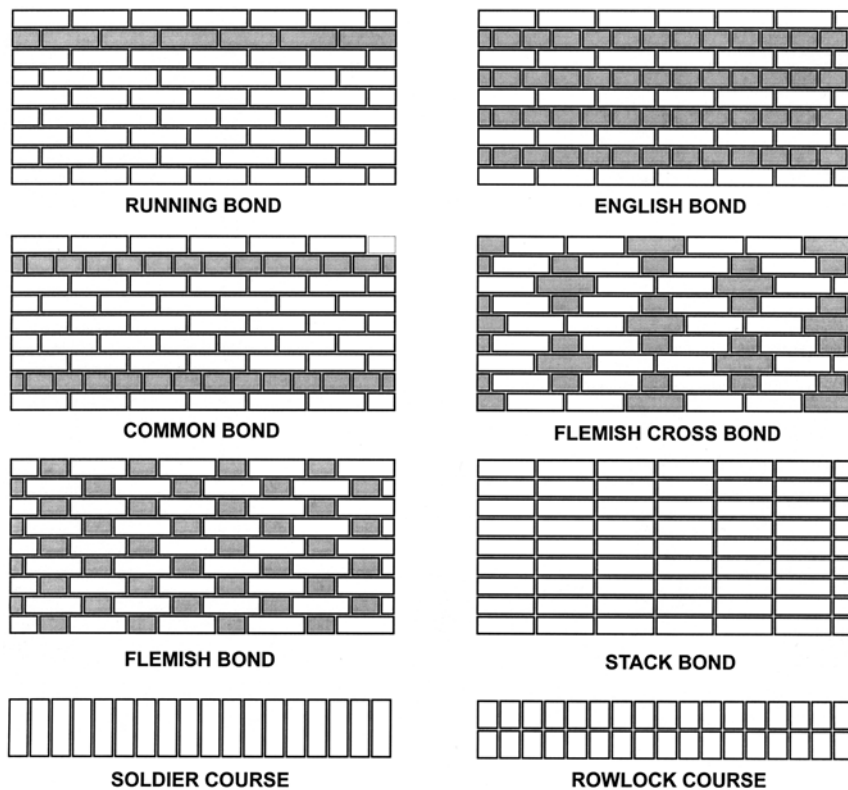
FIGURE 11.3. Brick Patterns.
