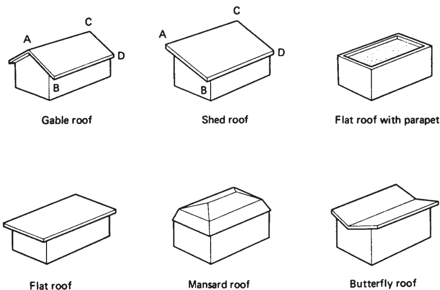
FIGURE 14.9. Typical Roof Shapes.
