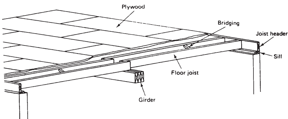
FIGURE 13.3. Floor Framing.
