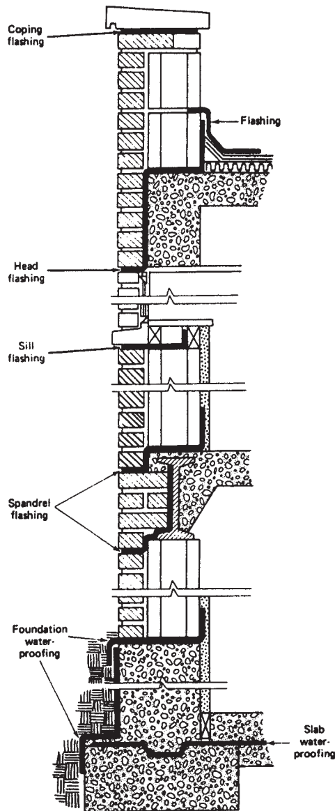
FIGURE 11.18. Flashing Location.
