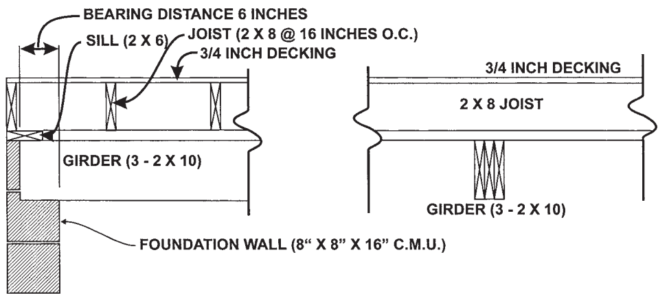
FIGURE 13.4. Bearing Distance.
