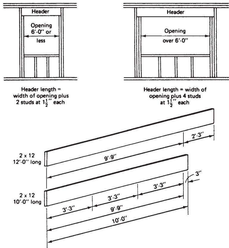
FIGURE 13.38. Header Example.
