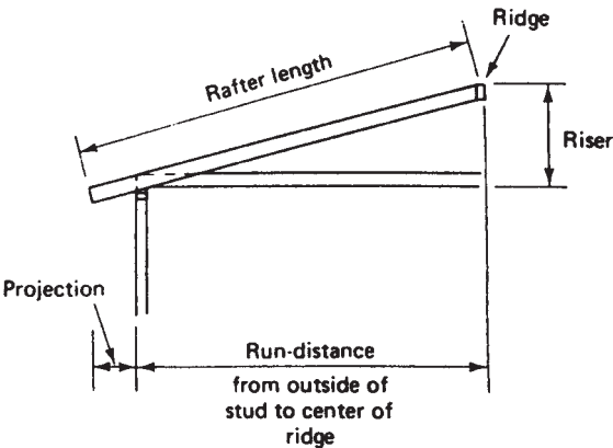
FIGURE 13.49. Rafter Length.
